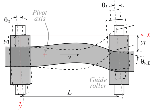
Figure 6 – Web span with remotely pivoted guide
