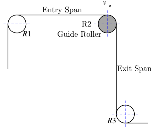
Figure 8 – Representation of two spans in a remotely pivoted guide for the simulation
