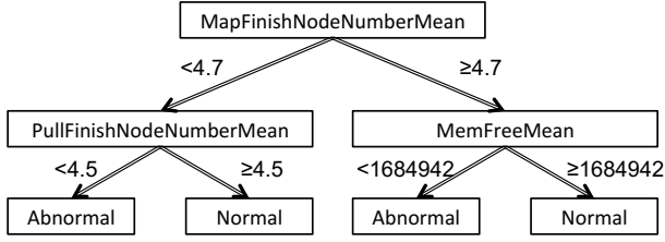
Figure 6: Model Generated by Decision Tree
