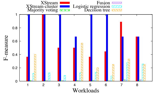
Figure 14: Consistency comparison
