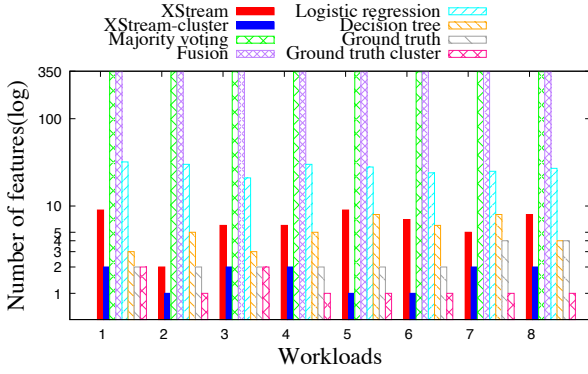
Figure 15: Conciseness comparison
