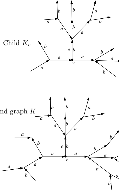
FIGURE 1. Child K_e of a round graph K of grade 3 with center v . Here N = 2 , F_2 = F(a, b) and \Gamma is the standard rose corresponding to the free basis \{a, b\} of F(a, b) .
