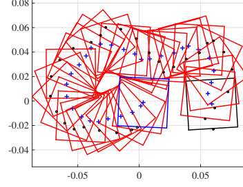
(b) Trajectory tracking with dynamic feedback linearization.
