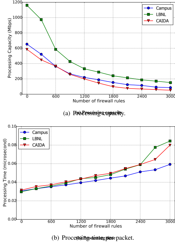
Fig. 7: Relationship between virtual firewall performance and rule size.
