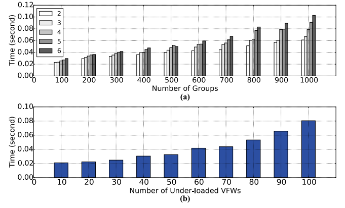
Fig. 10: Performance of provision plan calculation.
