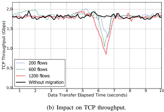
Fig. 9: Performance overhead of migration.
