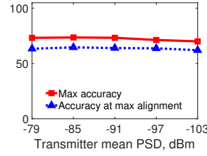
Fig. 6. Maximum and achieved accuracy with decreasing transmitter PSD. Alignment is a good proxy for accuracy across all PSD regimes. Achieved accuracy is high, persistent and close to the max accuracy.
