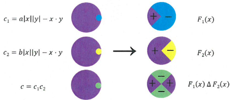
FIGURE 4. Other set operations yield even more examples of optimal transportation.
