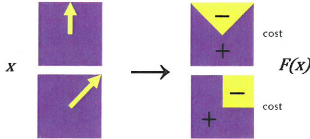
FIGURE 2. Optimal transportation F maps each x on a ray from the origin to a cone about that ray.
