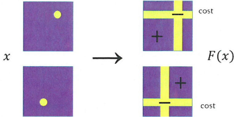
FIGURE 6. Optimal transportation on the flat rectangular torus maps each x to a small neighborhood around the coordinate axis centered at that point.
