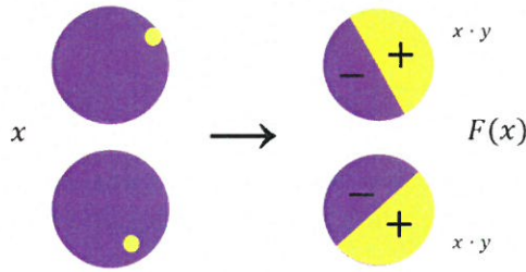
FIGURE 1. Optimal transportation F from the unit ball in \mathbf{R}^2 to itself with cost c(x, y) = (x - y)^2 and constraint h = 2 maps each x to the half-ball \{x \cdot y > 0\} .
