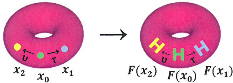
FIGURE 5. Optimal transportation F maps each x to an H -shaped region.
