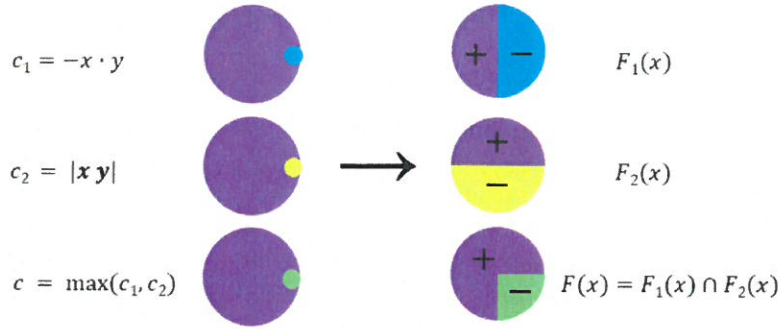
FIGURE 3. The intersection of optimal transportation plans yields a new optimal transportation plan under certain hypothesis.
