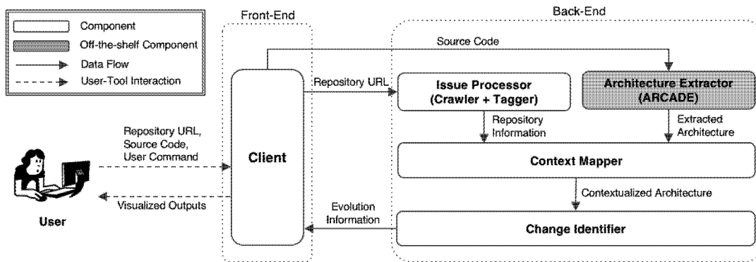
Figure 2: EVA's Architecture
