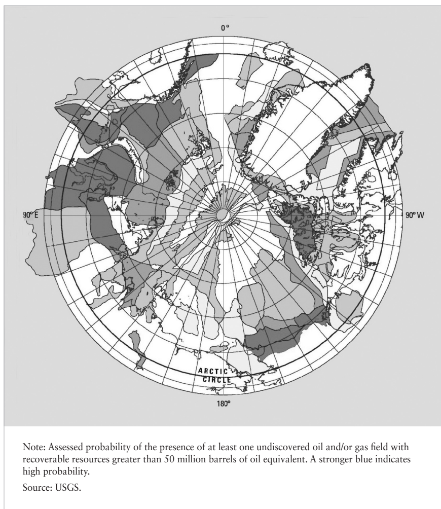
Figure II.5 Petroleum Potential in the Circum-Arctic
