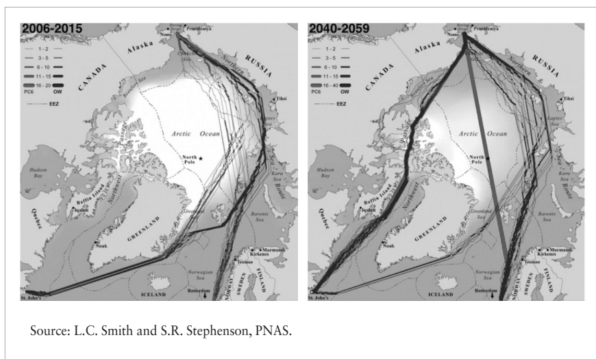
Figure II.4 Trans-Arctic Navigation Routes Today Versus Mid-Century
