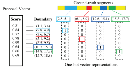
Figure 6: An example on converting ground-truth segments into one-hot vector representations from Proposal Vector.
