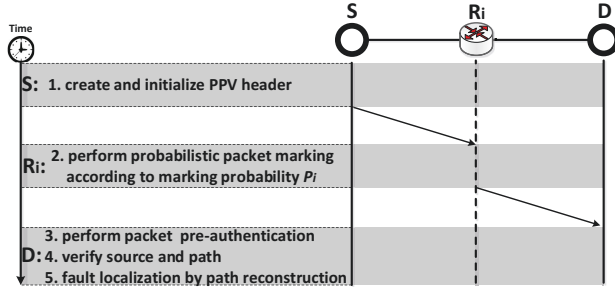
Fig. 2. The PPV overview when the packet is delivered through R_i towards D . Different entities handle the packets according to the responding rules.
