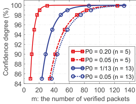
Fig. 5. The relationship between confidence degree C and the number of verified packets m with the average path length of AS or router level at D .
