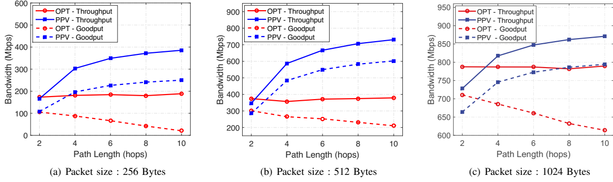
Fig. 6. The relationship between router's forwarding efficiency (throughput and goodput) and path length in the scenarios of different packet sizes.
