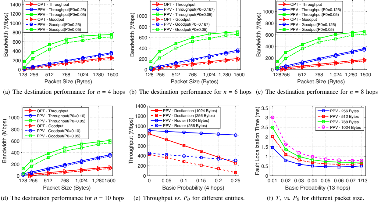
Fig. 7. The destination performance in terms of throughput, goodput and fault localization time with different packet sizes, path length and basic probabilities.
