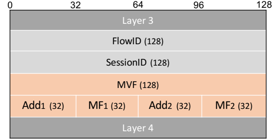
Fig. 3. The format of PPV header between Layer 3 and Layer 4 that contains seven fields and takes a fixed length of 64 bytes.
