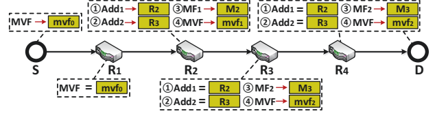
Fig. 4. An example of changing process of PPV header, where the red arrow denotes the dynamically update operation during packet delivery.
