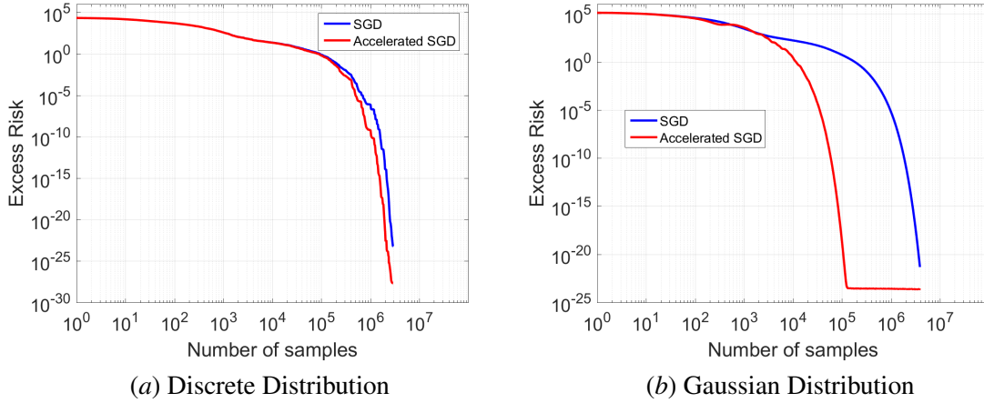
Figure 3: Comparison of averaged SGD with this paper’s accelerated SGD in the absence of noise ( \sigma^2 = 0 ) for the Discrete and Gaussian distributions with d = 50, \kappa \approx 10^5 . Acceleration yields substantial gains over averaged SGD for the Gaussian case, while degenerating to SGD’s behavior for the discrete case. See section 1.2 for discussion.
