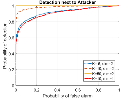
Fig. 1. ROCs temporal difference detection performance at the neighboring nodes of the attacker.
