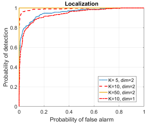
Fig. 2. ROCs temporal difference localization performance at the neighboring nodes of the attacker.
