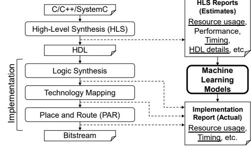
Figure 1: FPGA tool flow with HLS and proposed machine learning models (in bold) – The models use underlined metrics in the HLS reports to predict underlined post-implementation metrics.
