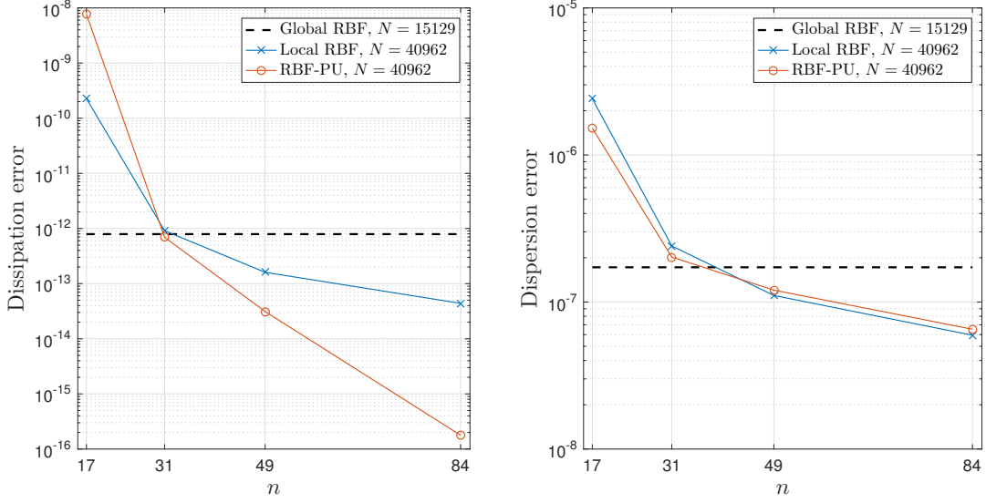
Figure 4: Relative dissipation (left) and dispersion (right) errors (13)–(14) for the solid body rotation of a cosine bell test case after one revolution as n increases in the local RBF and RBF-PU methods. The global RBF method does not have a dependence on n and is included as a dashed line for reference.
