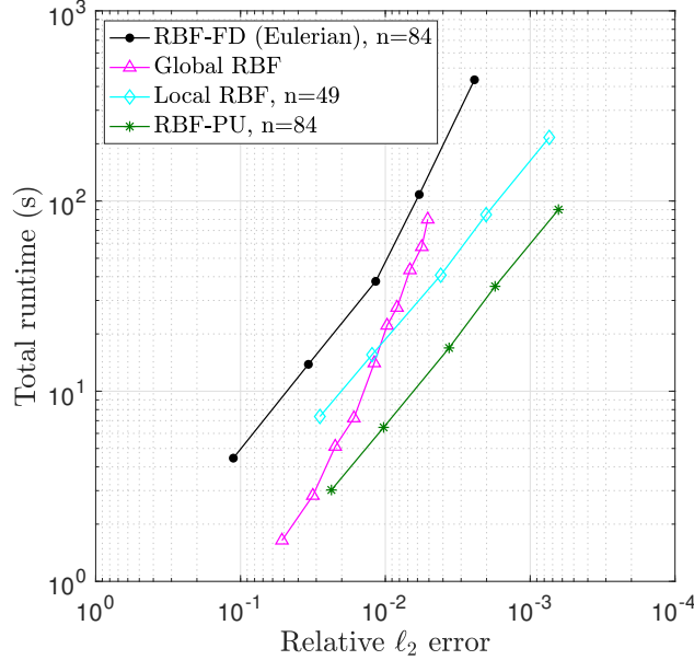
Figure 14: Comparison of the three new SL RBF schemes and the Eulerian RBF-FD scheme from [6]. The plot shows the computational cost (runtime) versus relative \ell_2 error for the Cosine Bells deformational flow test case. The stencil sizes for the global RBF, local RBF, RBF-PU, and Eulerian RBF-FD methods are shown in the legend. For the latter three methods, the same node sets were used of sizes N = 5762, 10242, 23042, 40962 , and 92162 .
