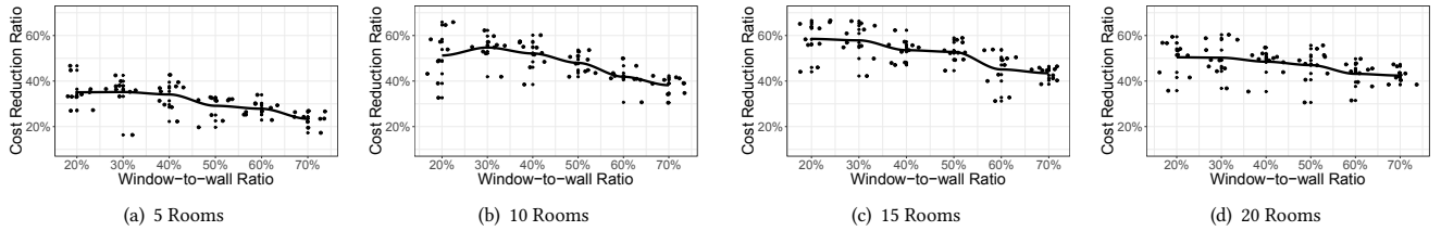
Figure 8: Cost reduction ratio with total number of rooms and window-to-wall ratio.
