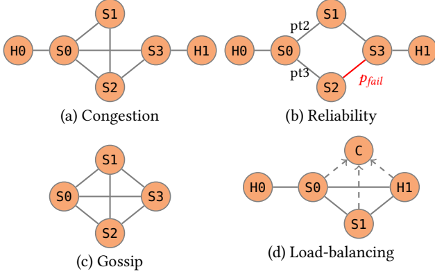
Figure 11. Network topologies used in our benchmarks
