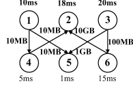
Figure 1: Example of a job DAG. Nodes represent tasks, with execution latency showed next to them. Edges represent flows and their sizes.
