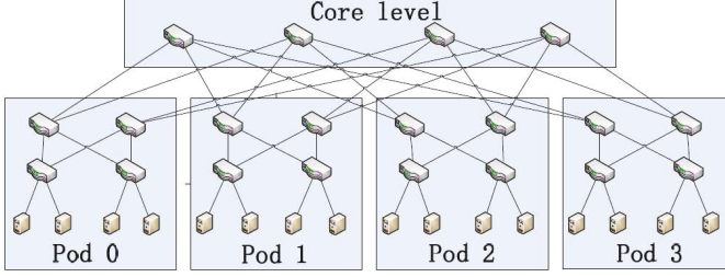
Figure 2: Fat tree topology.
