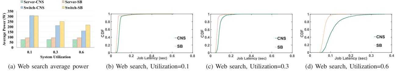
Figure 9: Average power and latency for 2000 Poisson-arrival web search jobs under low, medium, and high system utilization respectively. Suffix -CNS represents PopCorns framework and -SB denotes baseline Server-Balanced job scheduling algorithm.
