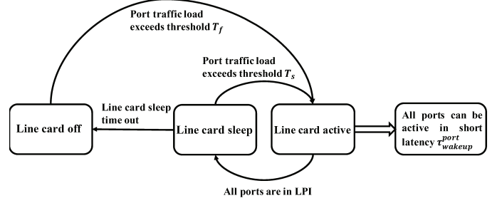
Figure 4: Power state transition overview.
