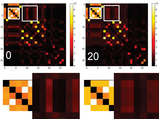
Figure 4: Two heat maps of 28 \times 28 similarity matrix S of nodes of C20N2O5S (Benfuracarb). One (labeled by 0) is before training, and the other is after the first 20 epoch. Enlarged part of matrix better indicates the learning of graph.
