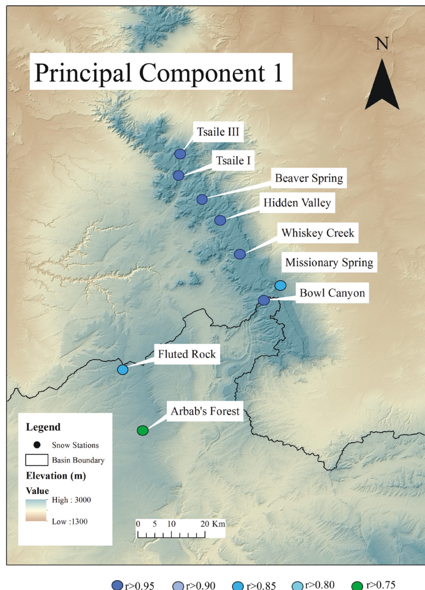
Figure 6. Year-to-year correlation map of March SWE for Principal Component 1.
