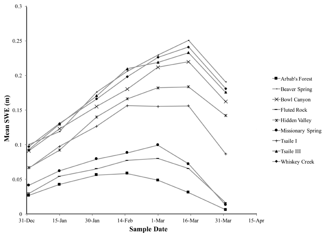
Figure 2. Climatological mean snow water equivalent (SWE) at each site, illustrating the seasonal cycle of snowpack for Navajo Nation snow survey sites.
