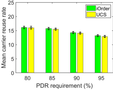
Fig. 18. Comparison with iOrder under the random topology
