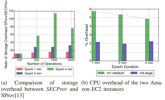
Fig. 5: CPU and storage overhead analysis
