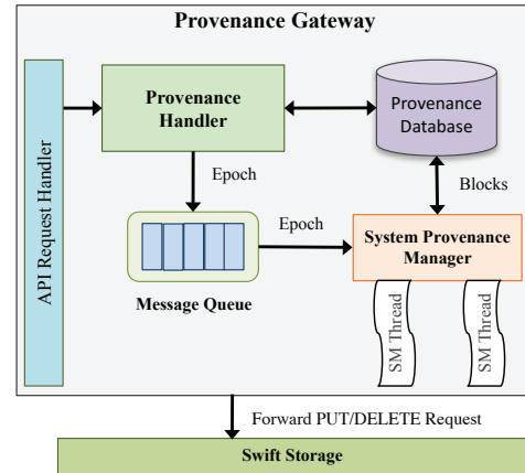
Fig. 3: Integration of SECPProv with Swift Storage
