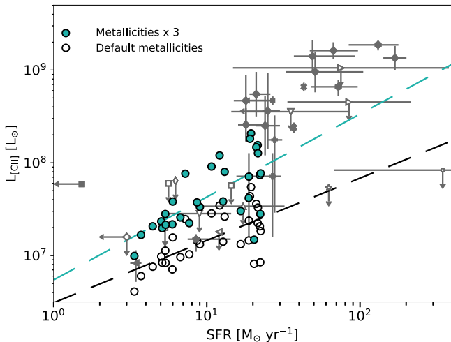
Figure 14. Effect of boosting the (default) metallicities of each fluid element in our simulations by a factor of three results in galaxy [C II] luminosities (filled green circles) that are on average \sim 2.5 – 3\times higher. Even so, this does not bring the simulations fully into accord with the [C II]-bright detections at z \simeq 6 , although there is an overlap with observations for some simulations. The dashed cyan line shows the log-linear fit to the simulations with high metallicities.
