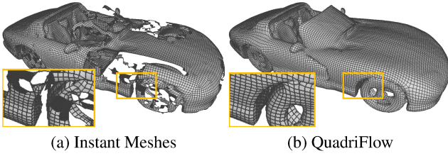
(a) Instant Meshes (b) QuadriFlow Figure 9: (a) Example where a nonmanifold input triangulation leads to an Instant Mesh with holes. (b) Because QuadriMesh removes inverted triangles from the position field representation, it produces a manifold mesh with the correct topology.
