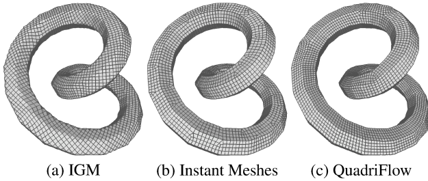
Figure 12: Surface quadrangulations of the model Knot1 using Integer-Grid Map (IGM) , Instant Meshes , and QuadriFlow . As we borrow the extrinsic energy formulation from Instant Meshes , our mesh edges are aligned with shape features, unlike IGM 's.
