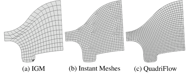
(a) IGM (b) Instant Meshes (c) QuadriFlow Figure 10: Quadrangulation of the model Fandisk using IGM, Instant Meshes, and QuadriFlow (our method). Our mesh has less angle distortion than IGM, and fewer vertices of irregular valence than Instant Meshes.
