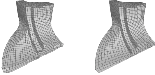
(a) Only tangential constraints (b) With sharp edge constraints Figure 8: (a) The tangent plane restriction does not suffice to preserve sharp edges. (b) Line constraints preserve sharp features better.
