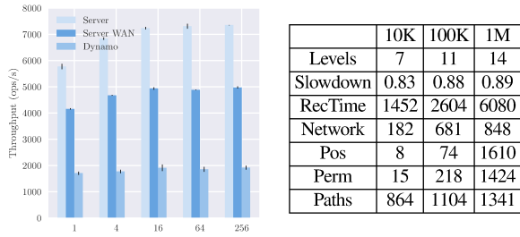
(a) Checkpoint Frequency (100K) (b) Server Wan Recovery Time (ms) Figure 11: Durability
