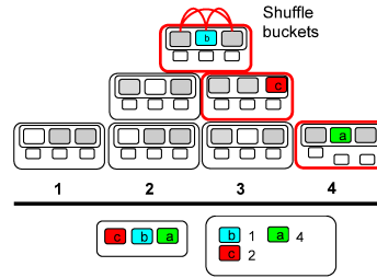
Figure 3: Eviction - Write Phase
