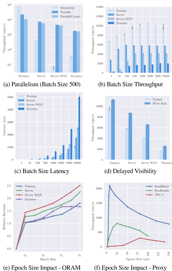
Figure 10: Performance impact of various features
