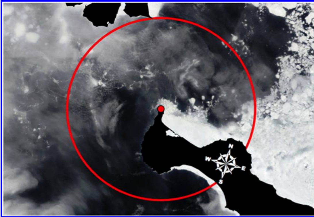
Fig. 12. 2 May 2318z true-color MODIS granule acquired by Terra at 250 m. The red circle and dot are the same as in Fig. 11. To the west and south of Gambell, in the upper left quadrant of the tile, sea ice in low concentration obscured by thin low-level stratoform clouds is visible in brighter white, geometric shapes. Landfast ice can be seen along the coastline to the east of the village and the south side of the island. To the north and east, ice in higher concentration is being compacted by westerly winds and south to north currents.
