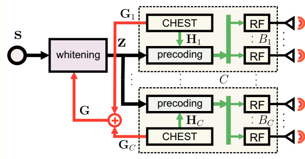
(a) Partially decentralized (PD) precoding architecture.
