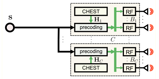
(b) Fully decentralized (FD) precoding architecture.
