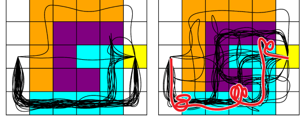
Figure 4: Left: Participant demonstrations in doing condition when only orange is dangerous. Right: Showing demonstrations with an example of extended behavior captured by the model of planning in observer belief space in red.
