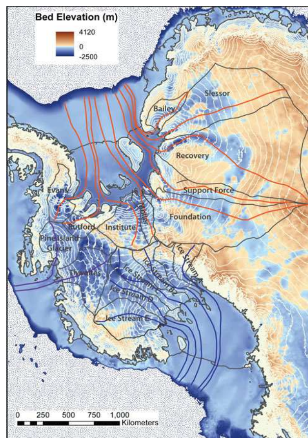
Fig. 1. Major West Antarctic ice-stream catchment areas, outlined in black (data from personal communication from I. Joughin). A characteristic flowline for each catchment area (from Byrd Polar Research Center, 1997) is overlain on Antarctica's bed elevation (Fretwell and others, 2013). Red flowlines drain to the Weddell Sea, purple to the Amundsen Sea and blue to the Ross Sea. The flowline routing beyond the present-day ice-shelf extent is drawn as a continuation of the flowline. Brown colors indicate elevations above the present-day sea level, and blue colors indicate elevations below sea level. Transition from solid to pixelated area marks the edge of the continental shelf.
