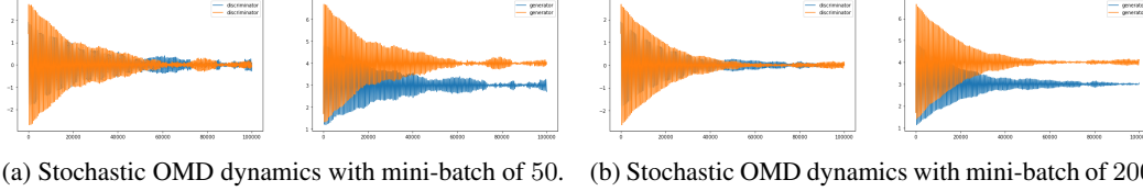
Figure 2: Robustness of last-iterate convergence of OMD to stochastic gradients.
