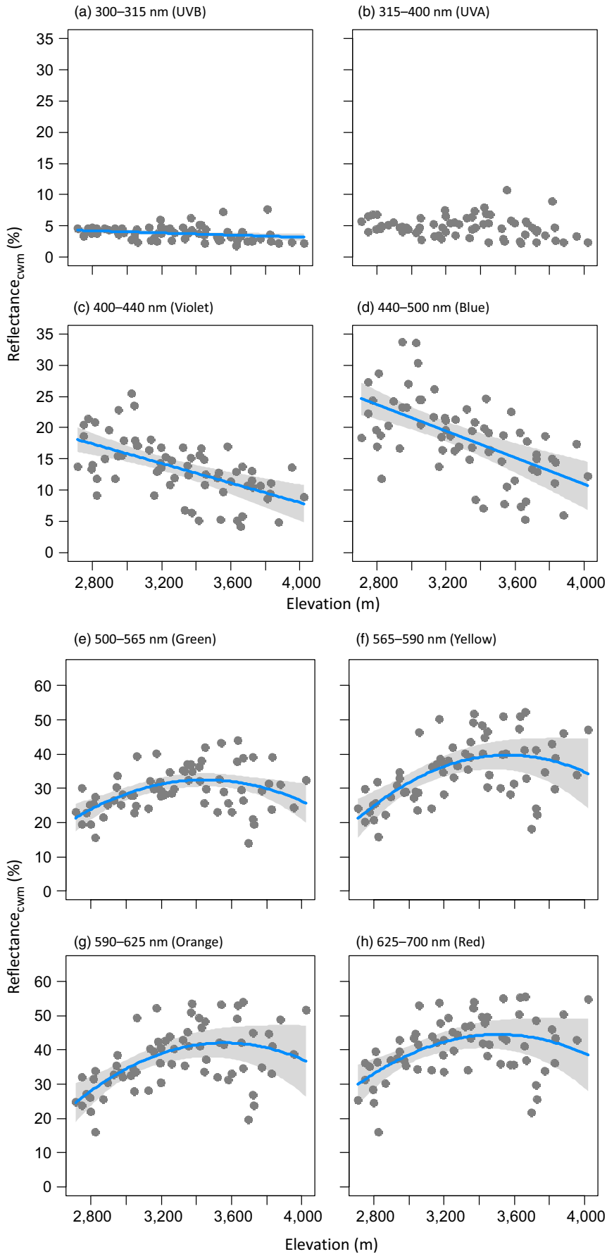
FIGURE 2 Raw spectra: relationships between elevation and floral reflectance cwm . The visible portion of the spectrum has been arbitrarily divided into eight spectral bands, each labeled by the hue as it appears in human vision (panels a–h). Each point represents the community-weighted mean reflectance in that band for a site. Conventions: lines and 95% confidence bands are plotted only when the best model included elevation. When the best model included transect, the plot is a partial leverage plot showing the effect of elevation after accounting for the random effect of transect.
