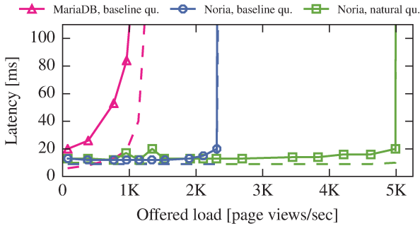
Figure 6: Noria scales Lobsters to a 5 \times higher load than MariaDB (2.3 \times with baseline queries) at sub-100ms 95%ile latency (dashed: median). MariaDB is limited by read computation, while Noria becomes write-bound.
