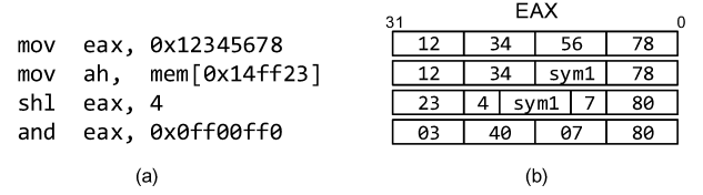
Figure 7: An example showing the states of multiple granularity symbolic execution.
