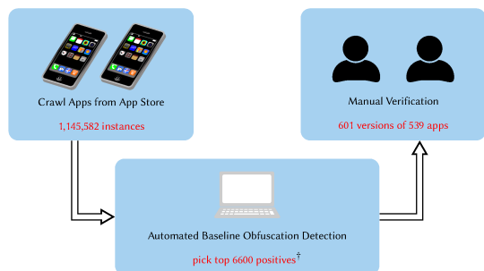
Figure 2: Workflow for sampling obfuscated iOS apps
