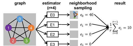
Figure 2: Approx. triangle count by neighborhood sampling
