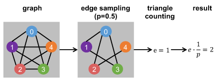
(a) Uniform edge sampling.
