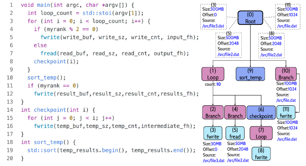
Fig. 3: PDG example.
