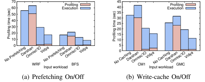
Fig. 8: Optimization
