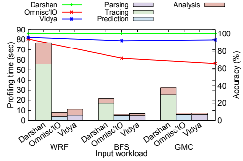
Fig. 7: Workflow Irregularity
