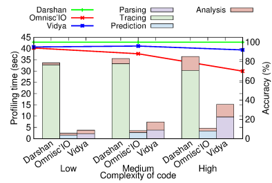
Fig. 5: Code Complexity
