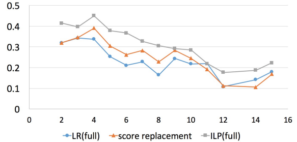
Figure 2: F1-scores on documents with different lengths. The x-axis indicates the number of sentences a document has. The y-axis indicates the macro average F1-score of causal relation identification.
