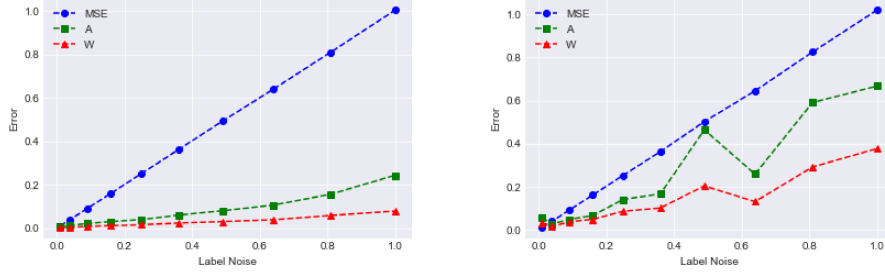
Figure 3: Error in recovering W , A and outputs (“MSE”) for different amounts of label noise. Each point is the result of averaging across five trials with 10,000 training samples, where for each trial W and A are both drawn as 10 \times 10 orthonormal matrices. The input distribution on the left is a spherical Gaussian and on the right a mixture of two Gaussians with one component based at the all-ones vector and the other component at its reflection.
