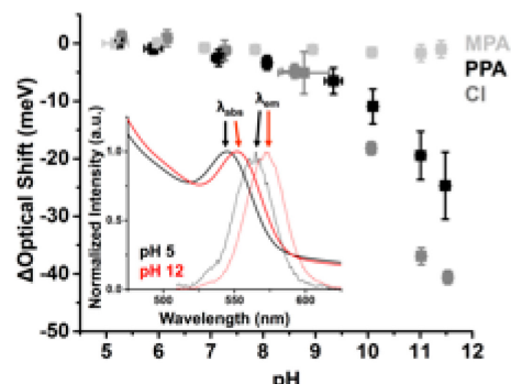
Figure 1 Shift of the excitonic energies of 0.7\text{ }\mu\text{M} CdSe QDs with 300 equivalents of MPA (light gray), 0.6\text{ }\mu\text{M} CdSe QDs with 300 equivalents of PPA (black) (see inset), or 0.6\text{ }\mu\text{M} CdSe QDs with 150 equivalents of HCl (dark gray) as a function of pH. Each data point is the the average of the shifts of the absorbance ( \lambda_{abs} ) and emission ( \lambda_{em} ) peaks within the optical spectra of at least three separately prepared samples of the QDs. The HCl-capped QDs were non-emissive (ESI † ), so data for those samples is collected only from absorbance spectra. The data at each pH value is from a separate sample.
