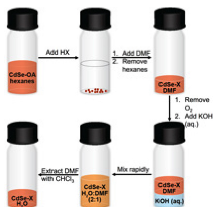
Scheme 1 The ligand-exchange/phase-transfer procedure. We add one of the three acids to as-synthesized oleate-capped QDs, followed by DMF addition and removal of hexanes. We add KOH (aq.) to the QDs under N_2 slowly, then mix rapidly and extract DMF with CHCl_3 .
