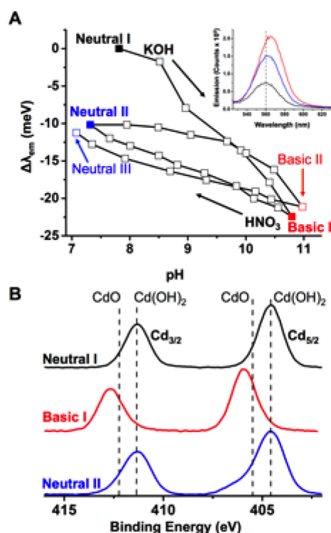
Figure 2 A) The \Delta\lambda_{em} of 1.0 \mu\text{M} CdSe with 300 equivalents of PPA during a pH cycling experiment in water using 0.1 M KOH and 0.1 M \text{HNO}_3 to adjust the pH. The inset shows the emission spectra at pH 8 (Neutral I), pH 11 (Basic I), and upon return to pH 7 (Neutral II). B) The average of three scans of the \text{Cd}_{5/2} and \text{Cd}_{3/2} regions of the X-ray photoelectron spectra of the CdSe/PPA system, deposited from a pH 7 solution (Neutral I, black), a pH 12 solution (Basic I, red), and upon bringing a solution back to pH 7 from pH 12 (Neutral II, blue). The dashed lines indicate the peak maxima for bulk \text{CdO} and \text{Cd(OH)}_2 (ESI † ).
