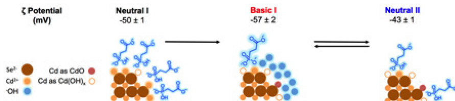
Figure 3 Top: \zeta potentials for a sample of 0.8 \mu\text{M} of CdSe QDs brought into water with 300 equivalents of PPA, at the three points in the titration labelled in Figure 2A. Bottom: schematic of the chemical processes at the surface of the QD as a function of pH consistent with optical, XPS, and \zeta -potential data on the CdSe/PPA aqueous system. Co-ions in the electrostatic double layer have been omitted for clarity.
