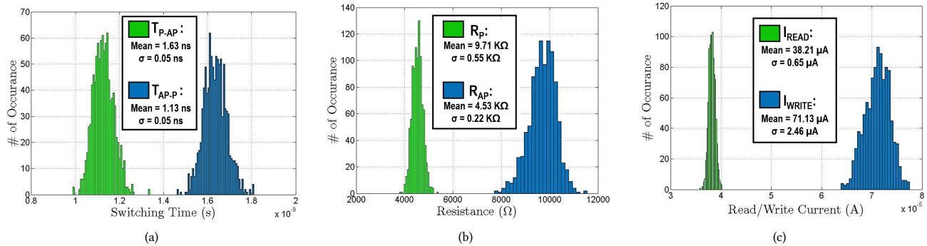
Figure 3: Simulation Results of 1,000 MC instances for (a) T_{P-AP} and T_{AP-P} Switching Times, (b) R_{AP} and R_P resistance states, and (c) read, I_{READ} , and write, I_{WRITE} currents.
