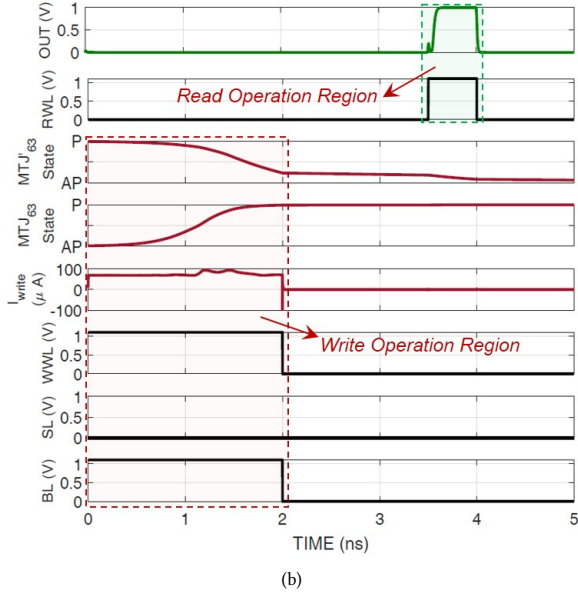
Figure 2: Transient response of C-LUT implementing 6-input OR operation for (a) ABCDEF = "000000" input signal, and (b) ABCDEF = "111111" input signal.
