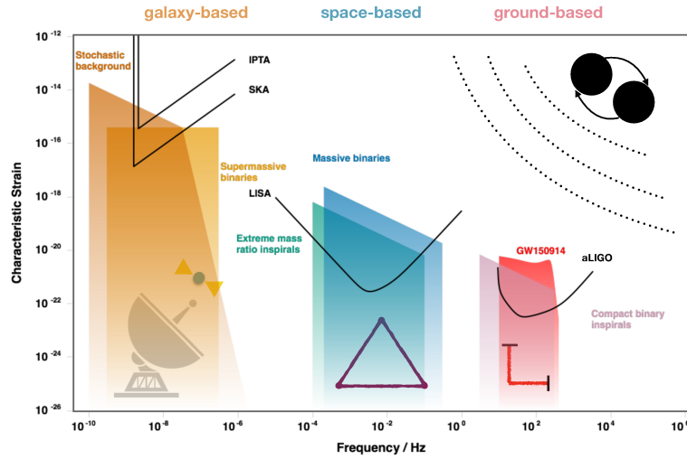
Figure 7. The spectrum of gravitational radiation from low-frequency (PTA) to high-frequency (LIGO). At very low frequencies pulsar timing arrays can detect both the GWB from supermassive black hole binaries, in the 10^8 - 10^{10} M_\odot range, as well as radiation from individual binary sources which are sufficiently strong. We assume 20 pulsars with 100 ns timing precision with a 15 year dataset for IPTA, and 100 pulsars timed for 20 years with 30 ns timing precision for SKA. Both estimates assume 14-day observation cadence. This Figure was reproduced with minor changes from [415], who in turn also used free software from [416].
