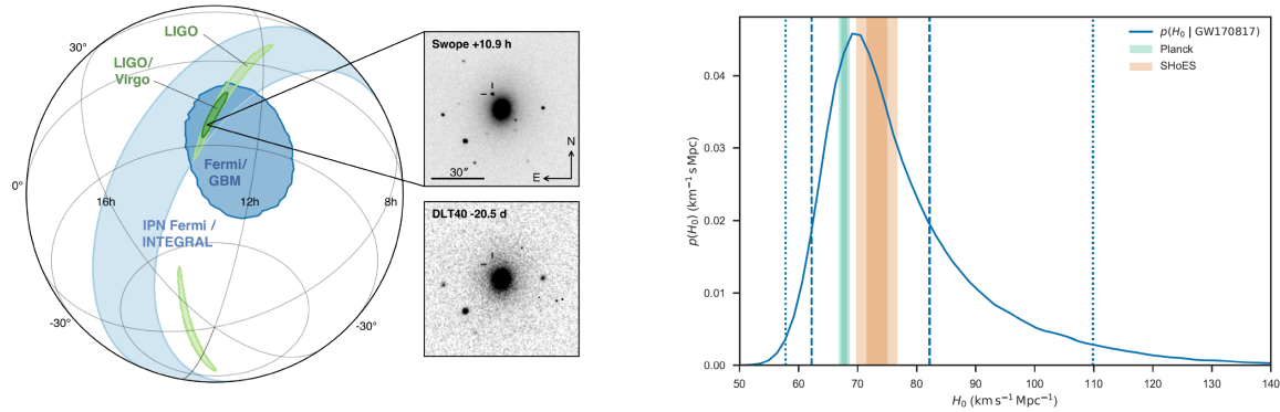
Figure 8. Left panel: The multi-messenger sky localization of GW170817 and the identification of the host galaxy. Right panel: The posterior distribution of H_0 compared to the recent CMB and SNIa constraints [639, 640]. Figures taken from Refs. [22, 24].
