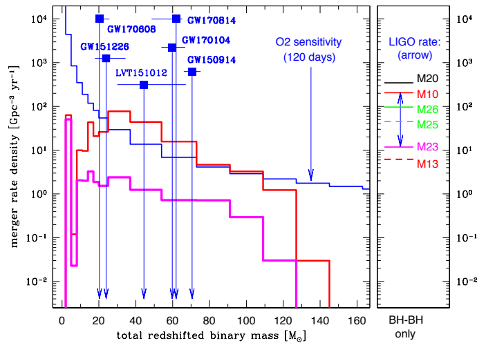
Figure 2. Left: Redshifted total merger mass distribution for two population synthesis models [123]: M10 (low BH natal kicks) and M23 (high BH natal kicks). The O2 LIGO sensitivity is marked; the most likely detections are expected when models are closest to the sensitivity curve. We also mark LIGO/Virgo BBH merger detections (vertical positions have no meaning), all of which fall within the most likely detection region between 20 – 100 M_{\odot} . Right: Source frame BBH merger-rate density of several population synthesis models for the local Universe ( z = 0 ). The current LIGO O1/O2 BBH merger rate is 12–213 \text{Gpc}^{-3} \text{yr}^{-1} (blue double-headed arrow). Note that the models with fallback-attenuated BH natal kicks (M10, M20) are at the LIGO upper limit, while models with high BH natal kicks are at the LIGO lower limit (M13, M23). Models with small (M26) and intermediate (M25) BH kicks fall near the middle of the LIGO estimate.
