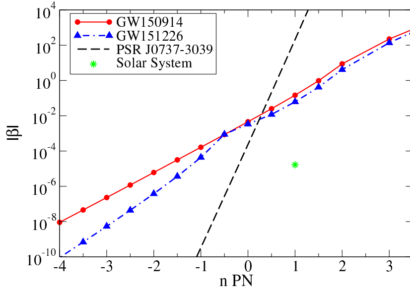
Figure 11. Upper bounds on the ppE parameter \beta with GW150914 and GW151226 entering at different PN orders. For comparison, we also present bounds from binary pulsar observations and Solar System experiments. This figure is taken and edited from [1506].
