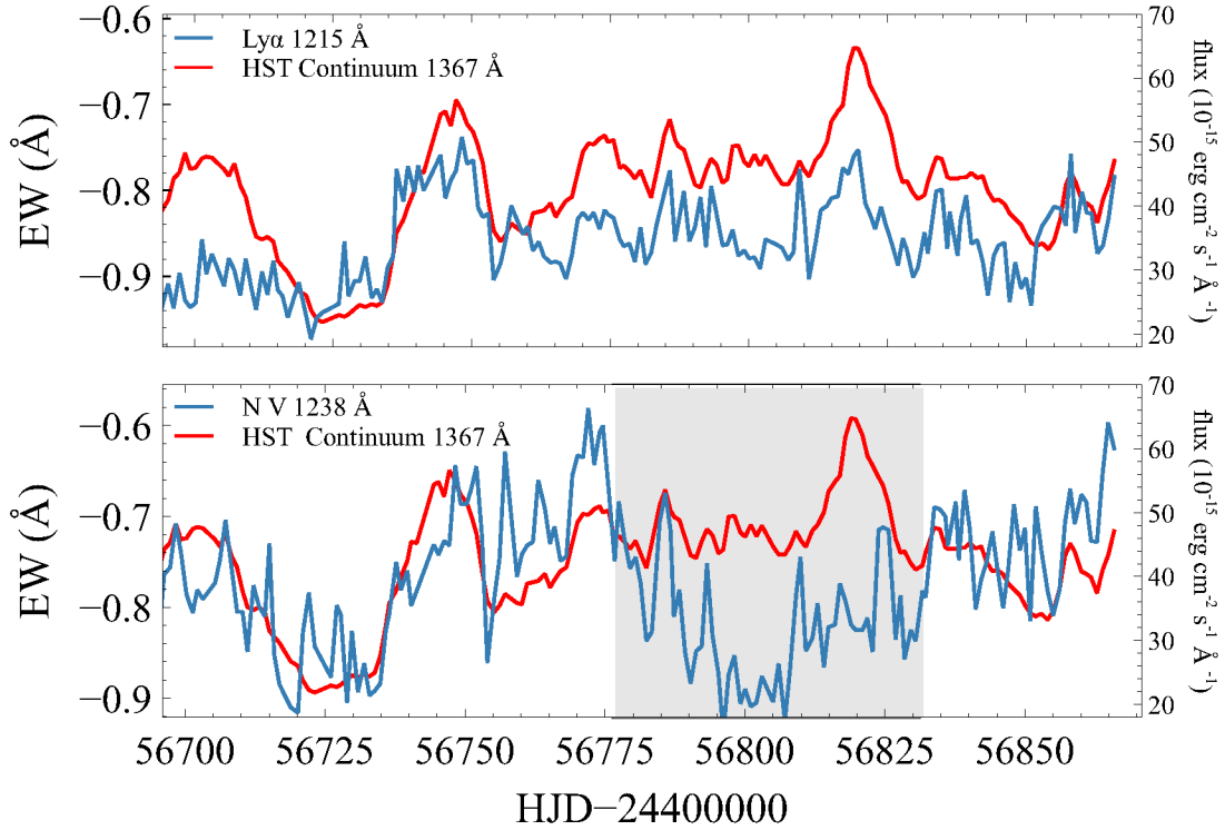
Figure 2. Both panels show the arbitrarily scaled FUV continuum in red, as a function of Heliocentric Julian Date -24400000 . The upper panel shows the equivalent width of the \text{Ly}\alpha absorber of Component 1 in blue and the lower panel shows the equivalent width of the corresponding \text{N V } \lambda 1238 absorption line. Shaded area indicates the time in which the “holiday” is happening.
