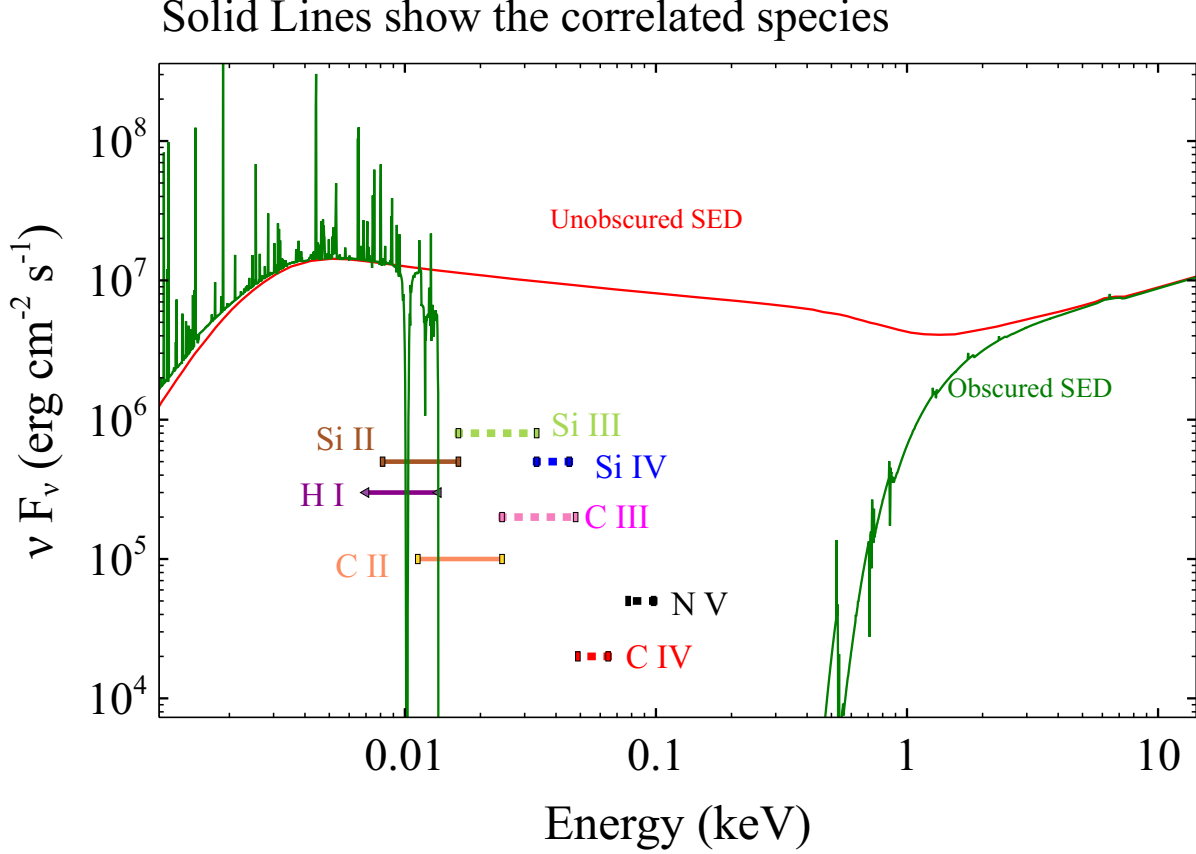
Figure 4. The expected SED transmitted through the obscurer and striking Component 1. Each line segment shows the energy required to produce the ion (left end) and to destroy the ion (right end). In this Figure, we assumed that the obscurer fully covers the continuum source. The column density to make the transmitted SED is N(\text{H}) = 1.2 \times 10^{22} \text{ cm}^{-2}
