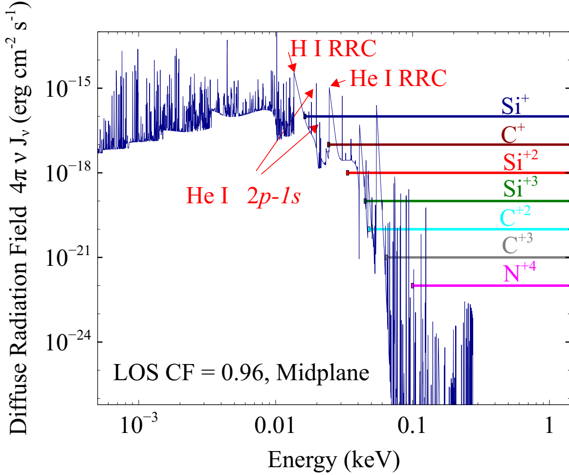
Figure 9. Diffuse emission field at the midplane of Component 1 with 96% obscuration. The left terminus of the horizontal lines shows the minimum energy needed to destroy the ion and produce the higher stage ion. RRC stands for radiative recombination continua and H I RRC is the Lyman continuum emission
