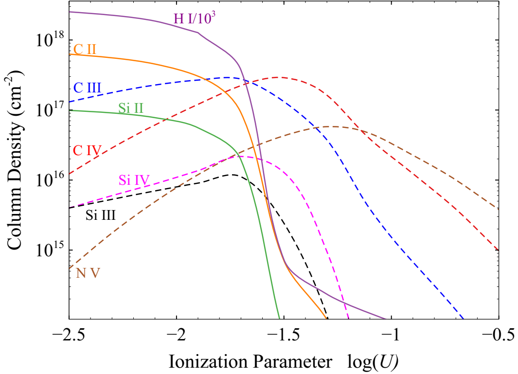
Figure 5. This shows how Component 1 column densities change as the ionization parameter changes. The hydrogen column density is divided by 1000 for comparison purposes. The solid lines are correlated species while the dashed lines are decorrelated. These changes are unlike those seen in the holiday, ruling out changes in U alone as the reason for the holiday.
