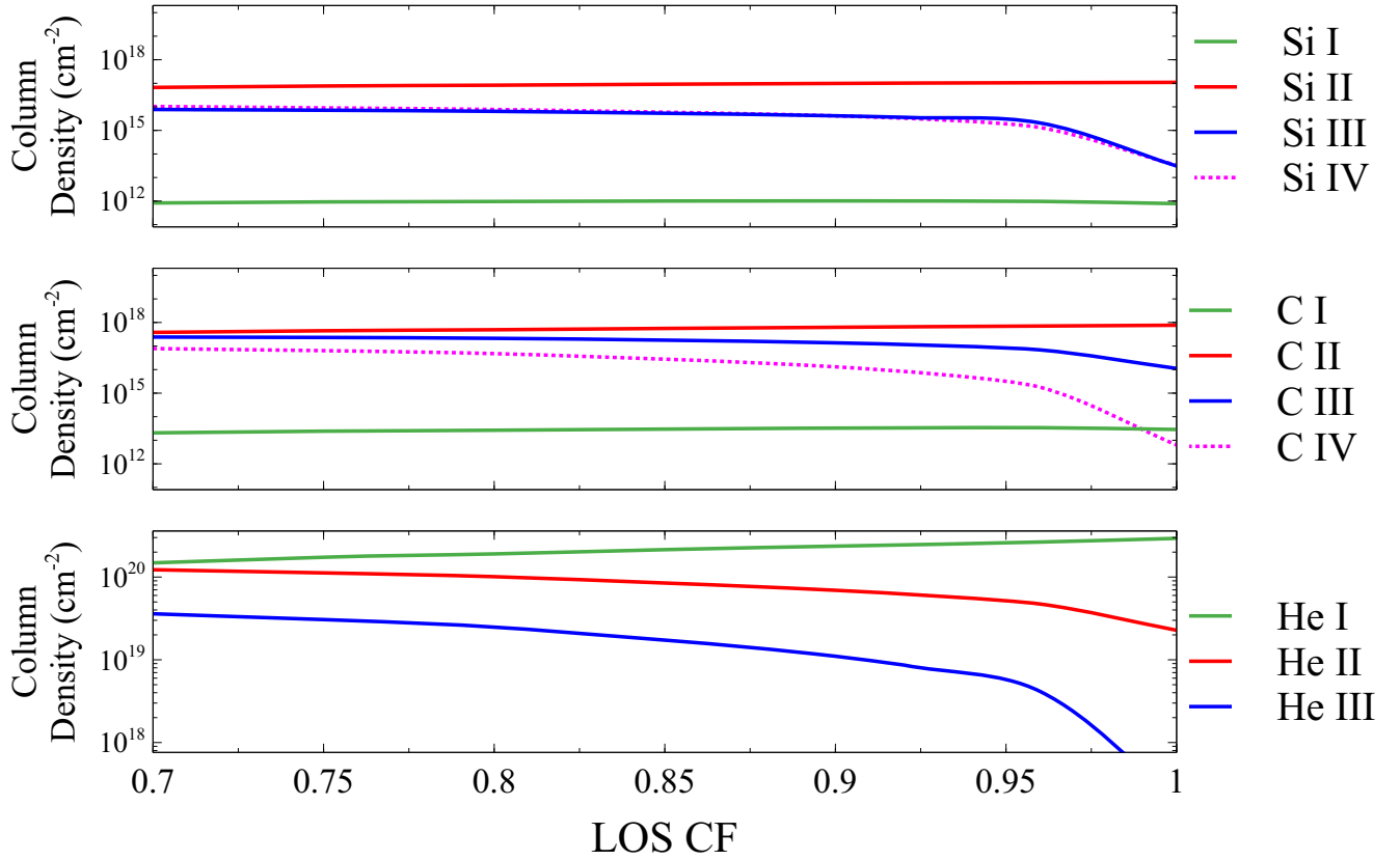
Figure 8. Variations of the column densities of different ionization stages as the obscurer LOS CF changes. Si, C, and He are shown in three panels, from top to bottom, respectively.
