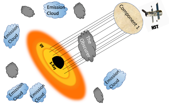
Figure 1. The geometry of the emission and absorption components discussed in this paper. The line of sight obscurer covers 70% to 100% of the X-ray source (Mehdipour et al. 2016). The gray clouds show other possible obscurers. These will be discussed in the next paper in this series. The blue blobs indicate the BLR clouds surrounding the source. Component 1, the narrow absorption line component with the highest outflow velocity ( -1165 \text{ km s}^{-1} ), is also shown. Component 1 is the absorbing component studied in this paper.
