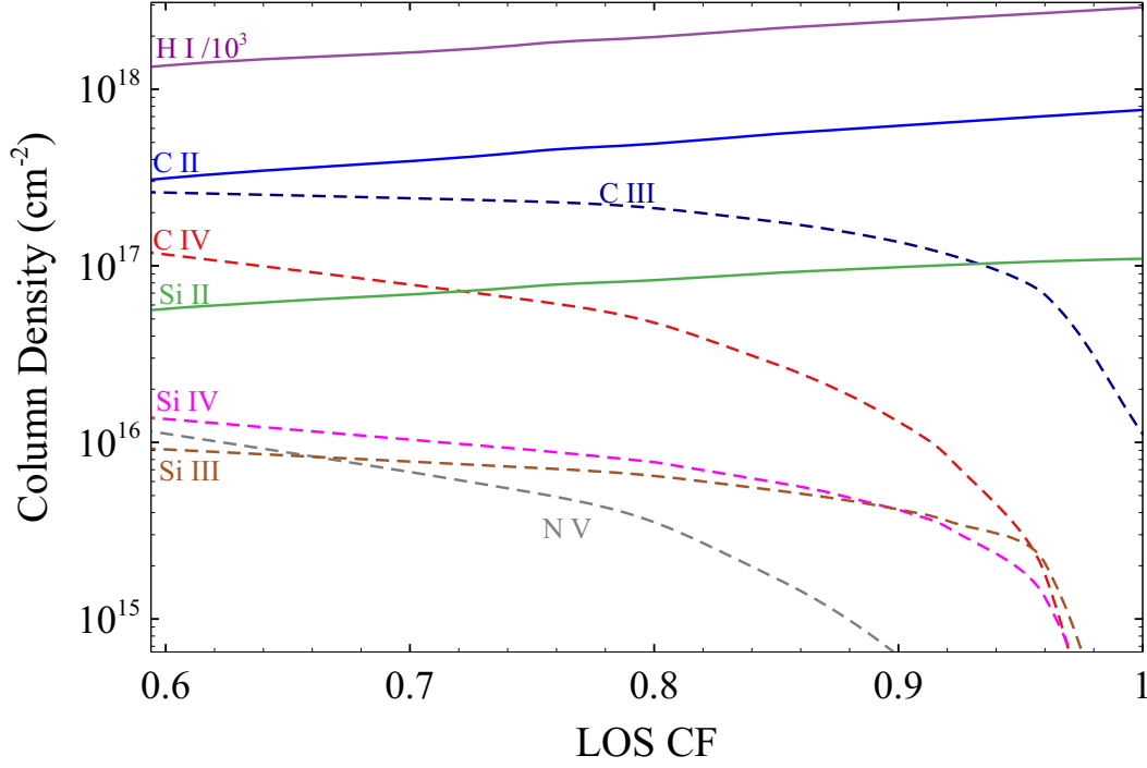
Figure 7. The effects of changes in the obscurer LOS CF upon the column densities observed by HST . Low-ionization species (solid lines) remained correlated while high ionization (dashed) species were decorrelated during the holiday, as expected from changes in the obscurer covering factor. The ionization parameters adopted for the obscurer and Component 1 are \log \xi = -1.2 ( \text{erg cm s}^{-1} ) and \log U = -1.5 , respectively.
