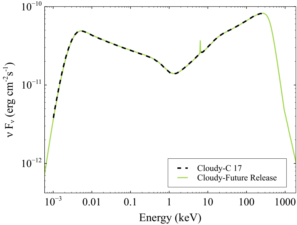
Figure 3. The intrinsic (unobscured) SED available in version 17 of cloudy (C17) is shown in dashed-style black line. It was zero outside the indicated range. The green line shows the improved SED (Mehdipour et al. (2015)) which will be implemented in future versions of cloudy .
