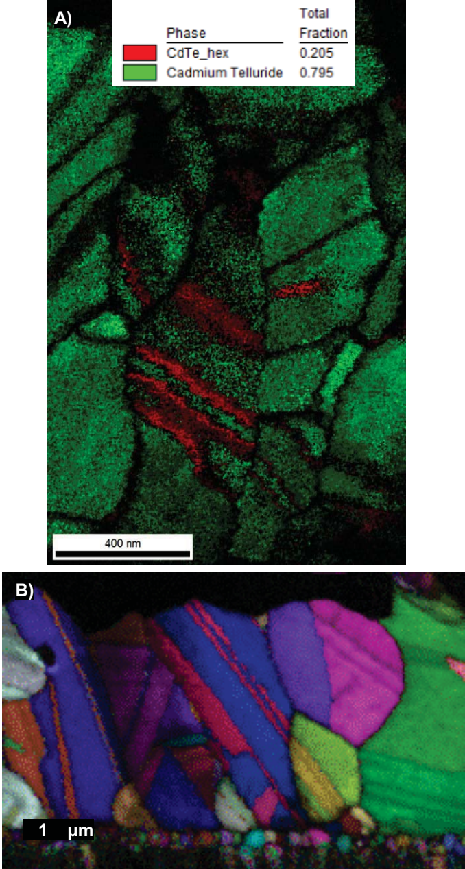
Fig. 8. EBSD derived maps showing a) phase/confidence index of an untreated CdTe cell b) inverse pole figure map of a treated device.
