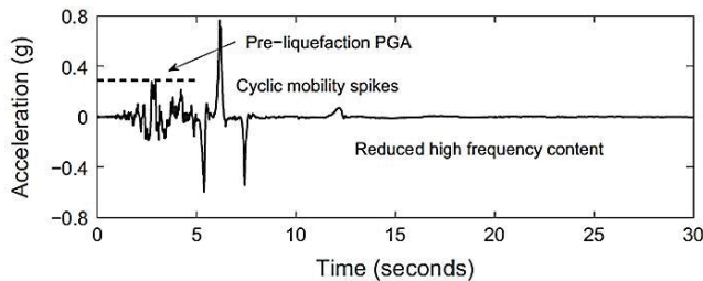
Figure 1. Ground motion record at NNBS during the M_w 6.2 Christchurch earthquake showing cyclic mobility/dilation spikes and the pre-liquefaction PGA (Wotherspoon et al. 2015).
