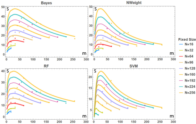
Fig. 10: Fixed-size dimension
