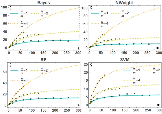
Fig. 9: Fixed-time dimension
