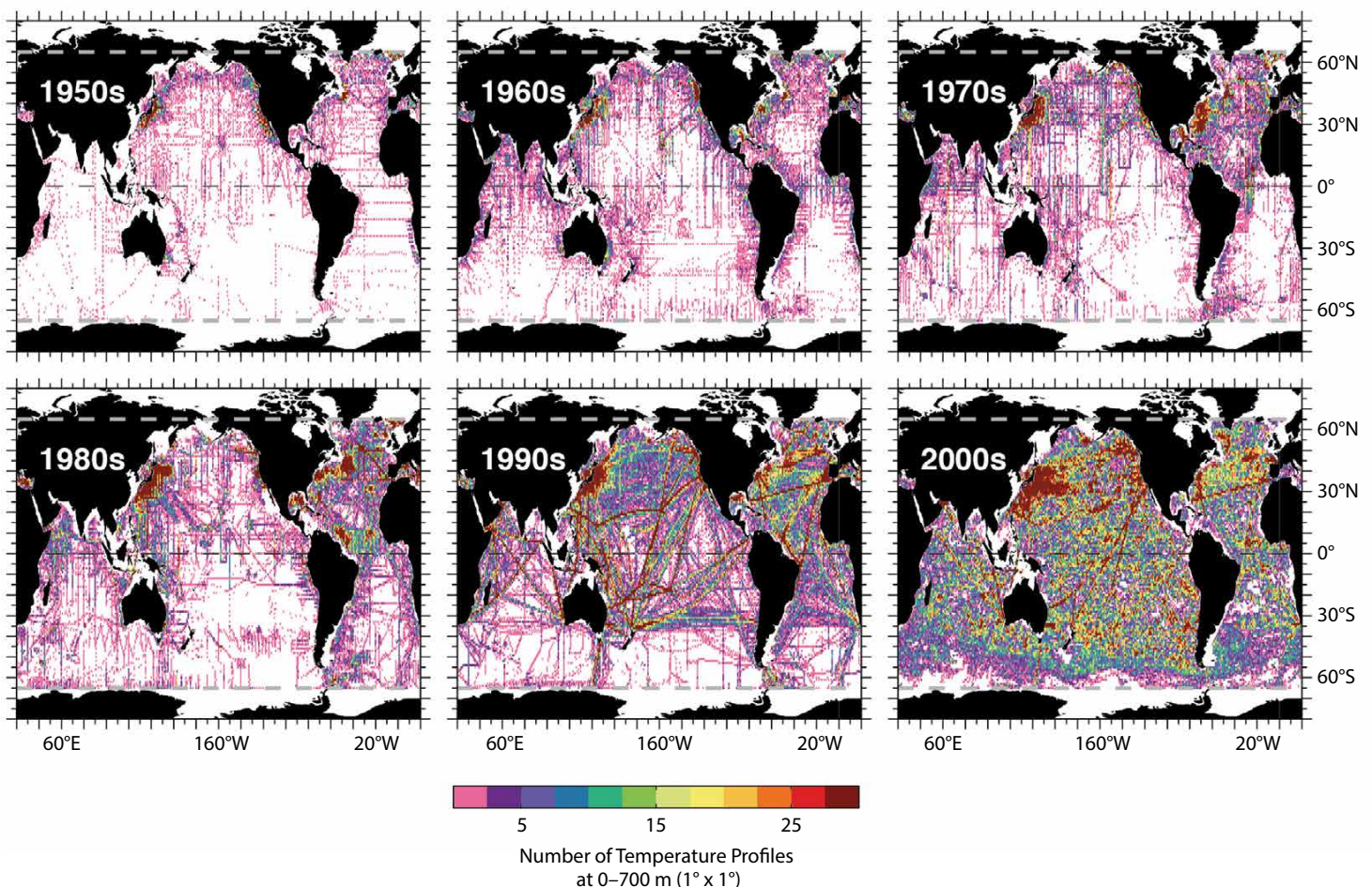
Figure 1. Historical coverage of upper-ocean temperature profiles in each decade since the 1950s. The drastic changes in the 2000s, especially in the Southern Hemisphere, are due to the advent of the Argo array of autonomous profiling floats. From Rhein et al. (2013)
