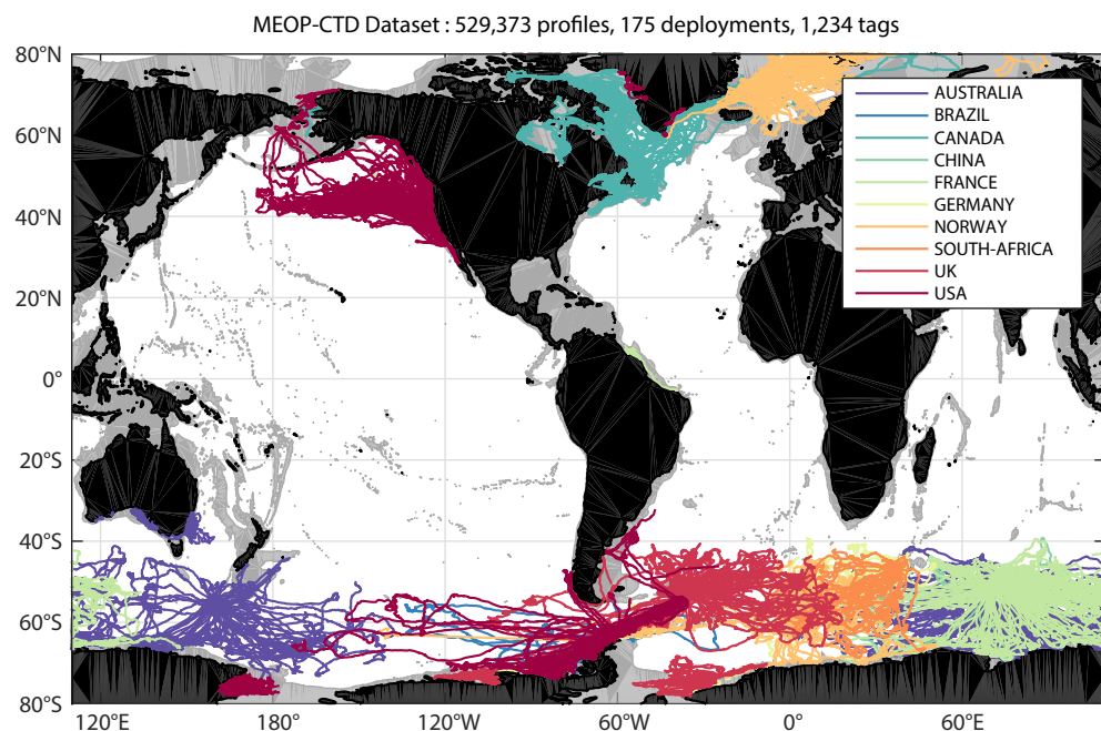
Figure 2. World map showing the 1,200 tracks currently available in the MEOP-CTD database, representing 530,000 hydrographic profiles (July 2016 version). See http://meop.net for more information on the data portal.
