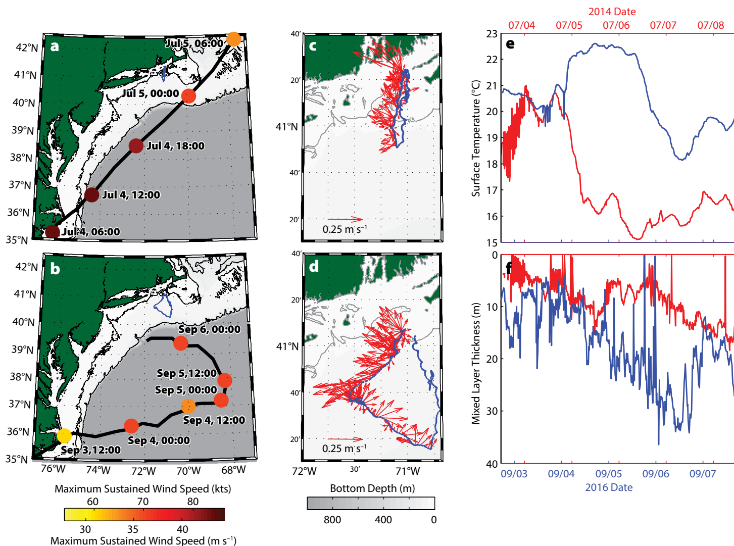
Figure 3. Glider observations of the effects of Hurricanes Arthur (2014) and Hermine (2016) in the Middle Atlantic Bight. Tracks of (a) Arthur and (b) Hermine with maximum sustained winds indicated by colors and tracks (blue) of Woods Hole Oceanographic Institution-operated gliders deployed in response to the storms. (c–d) Vertically averaged currents measured by the gliders before, during, and after the storms as the gliders moved offshore; only Hermine generated inertial oscillations (d). Time series of (e) surface temperatures and (f) mixed layer thicknesses measured by the gliders during Arthur (red) and Hermine (blue). From Goni et al. (2017)
