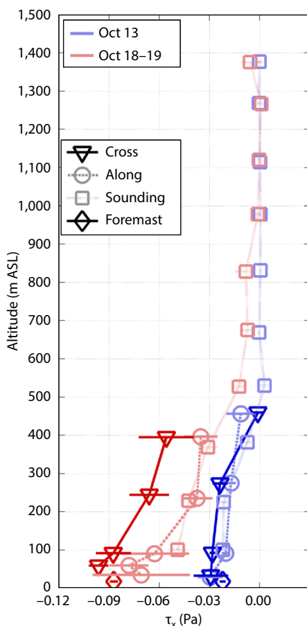
Figure 3. Vertical profiles of momentum flux in the marine atmospheric boundary layer, as measured by a turbulence probe on a ScanEagle. From Reineman et al. (2016)
