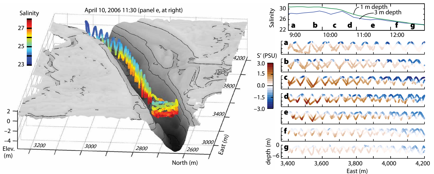
Figure 2. Repeat transects of salinity structure taken with a REMUS 100 during ebb tide in Elkhorn Slough, California, highlight the ability of autonomous underwater vehicles to operate in complex, energetic coastal environments. (left panel) Salinity observations mapped onto vehicle location, during transect in panel (e). (right panels) Time evolution of salinity deviation from mean transect salinity, S' = S - \text{mean}(S) . Time of transects is shown in top panel, with moored salinity traces from 1 m and 3 m depth.
