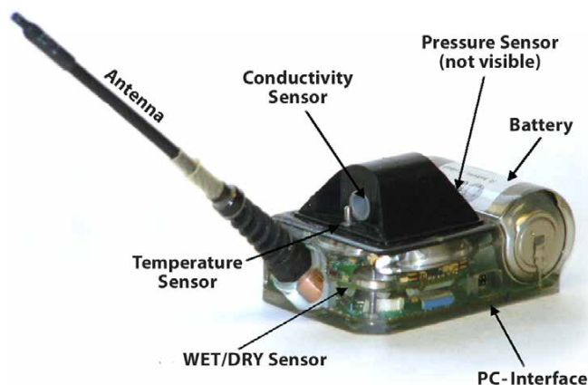
Figure 3. Photograph of a CTD-SRDL, with visible hardware components labeled (photograph by Lars Boehme, SMRU). The tag is potted in epoxy rated to 2000 m depth. Standard sensors include a CTD unit manufactured by Valeport Ltd (Devon, UK). The tag has a PC interface, is powered by a primary cell (battery) and has a telemetry option (ARGOS, GSM, UHF). From Photopoulou et al. (2015)
