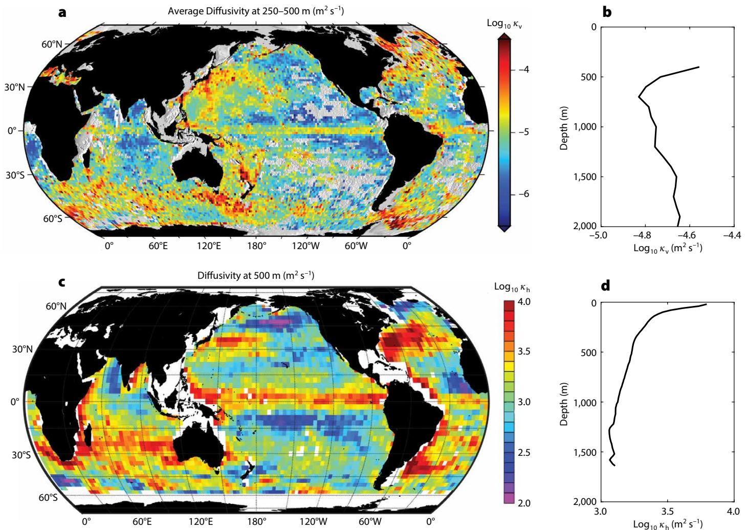
Figure 1. (a) Map, and (b) globally averaged profile of vertical diffusivity from Argo float temperature and salinity profiles (adapted from Whalen et al., 2012, with data updated through June 2016). (c) Map at 500 m depth, and (d) globally averaged profile of horizontal eddy diffusivity derived from Argo float temperature and salinity profiles and ECCO-2 eddy kinetic energy (adapted from Cole et al., 2015, with data updated to cover 2005–2015). Global averages are shown at depths with sufficient data.
