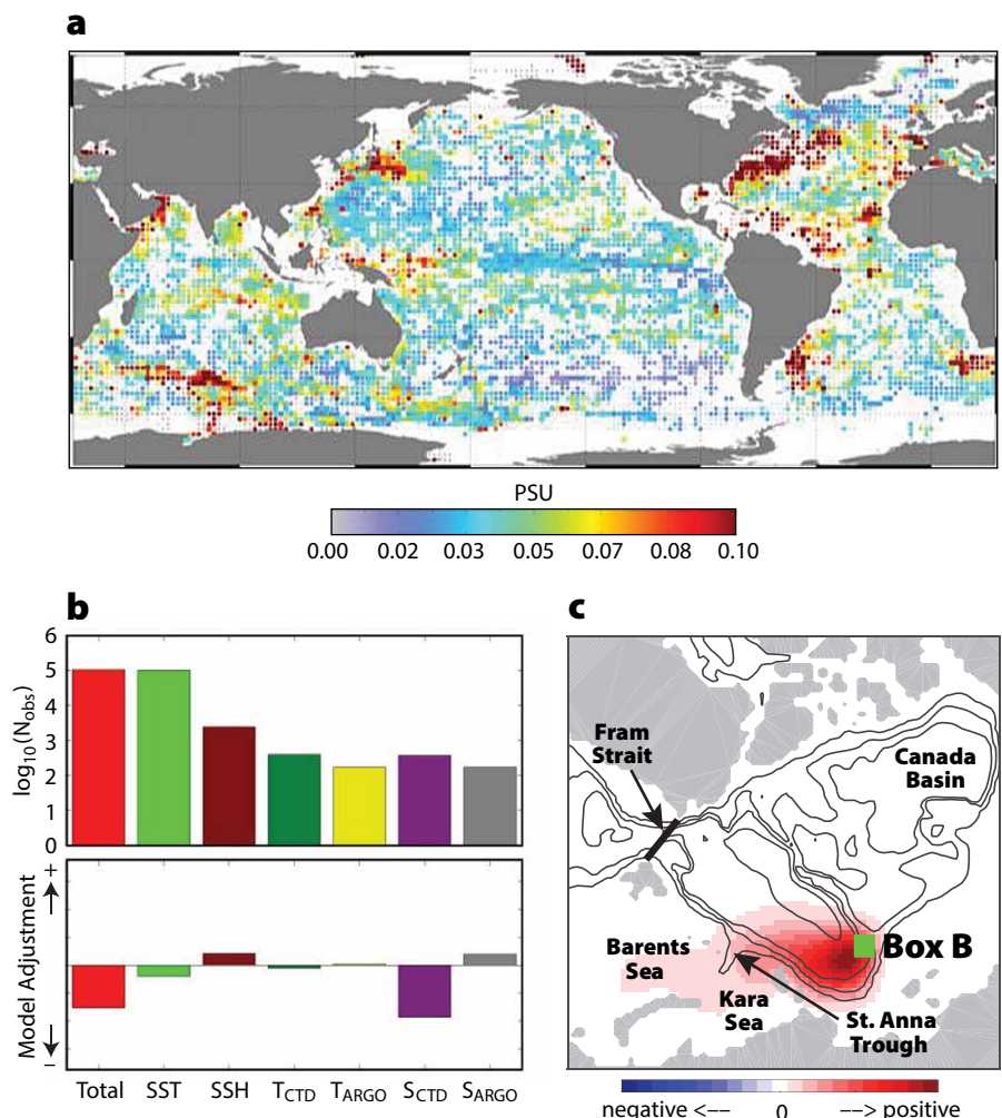
Figure 2. (a) Large misfits in salinity between a data constrained DA system and Argo float data over depth range 300–2000 m [subfigure adapted from Turpin et al. (2016)], (b) number of observations (upper) and impact of observations on the total adjustment (lower) during a 7-day assimilation in a California Current ocean data assimilation framework [subfigure adapted from Moore et al. (2011c)], (c) sensitivity of box B mean temperature at depth ~150 m to ocean salinity at depth 125 m up- and down-stream. Figure adapted from Nguyen et al. (2017)
