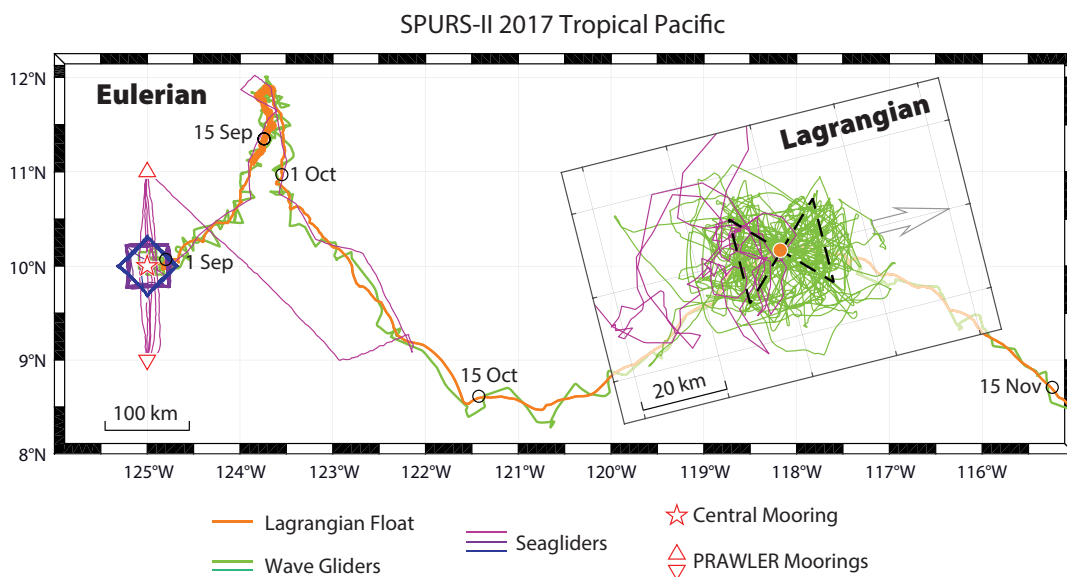
Figure 3. Experimental design for the autonomous components of the SPURS-II program shows a combination of Eulerian and Lagrangian components (from Lindstrom et al., 2017). A central mooring (star) provides intensive Eulerian measurements; Seagliders and Wave Gliders survey around it. A Lagrangian float (orange), launched at the mooring, is advected eastward in the strong currents and provides a reference point for a Seaglider (purple) and Wave Glider (green) surveying around it. The inset figure, rotated to align to the direction of the float drift, shows the Seaglider and Wave Glider trajectories relative to the float. A region approximately 20 km around the float is surveyed every few days. This design addresses the central goal of SPURS-II, which is understanding the salinity dynamics in this region by measuring both Eulerian and nearly Lagrangian time series and the spatial context of both.
