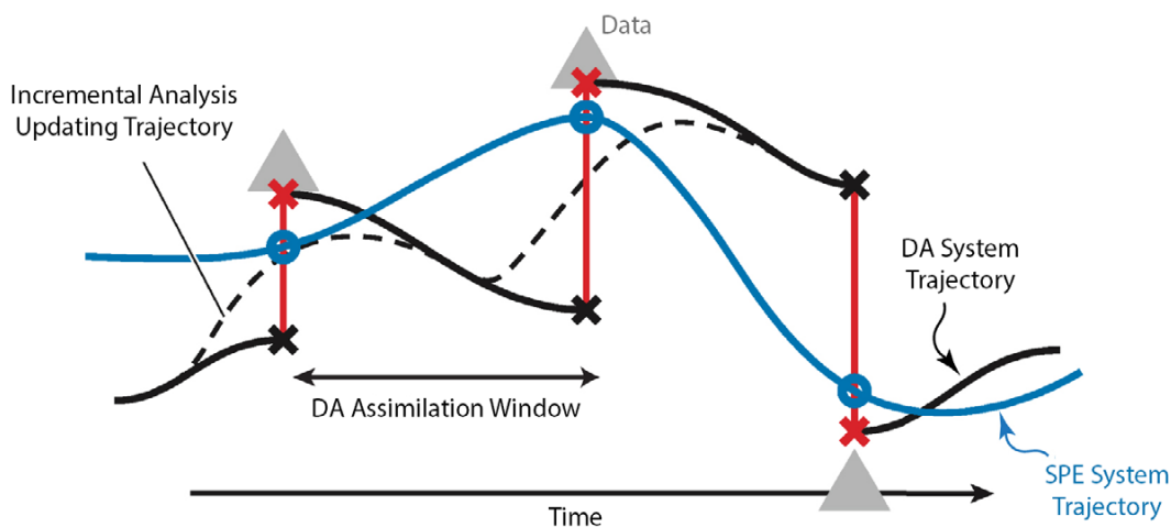
Figure 1. Schematic difference between data assimilation (DA) and state and parameter estimation (SPE) systems. Trajectories of DA and SPE systems are depicted with solid black and blue lines, respectively. In a DA system, at the end of each DA assimilation window, the model trajectory can lead to an ocean state (black cross) that diverges from observations (gray triangle), and a correction (re-initialization) can bring the model toward the observation (to within pre-defined criteria, red cross). Unphysical “discontinuities” can potentially be introduced in this correction step (red vertical lines) and can be mitigated through incremental adjustments (dashed black line), though the resultant smooth solution can remain dynamically unbalanced. SPE system trajectory (blue solid line) matches observations to within a pre-defined uncertainty range and guarantees conservation of heat, salt, and momentum over the entire estimation period. Figure adapted from Stammer et al. (2016)
