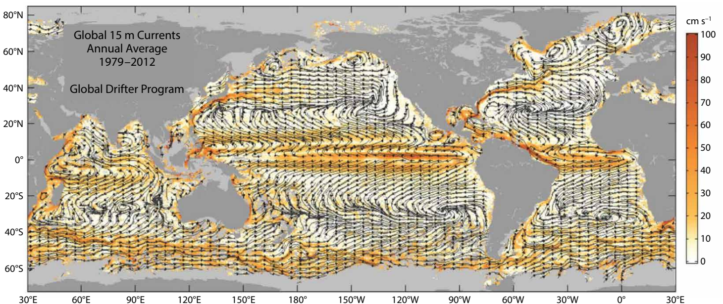
Figure 1. Mean current speeds (colors) from Global Drifter Program trajectories with streamlines (black lines). Adapted from Lumpkin and Johnson (2013)
