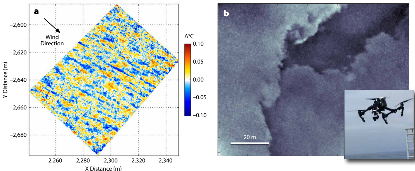
Figure 2. (a) Sample infrared imagery from a FLIR A325 aboard a ScanEagle (adapted from Reineman et al., 2013) showing Langmuir-like surface signatures aligned with the wind. (b) Uncalibrated test image from a FLIR-DJI ZenmuseXT aboard a small DJI Inspire 1 quadcopter (inset) showing a temperature front (A.F. Waterhouse, E. Lo, and D. Rissolo, pers. comm. ).
