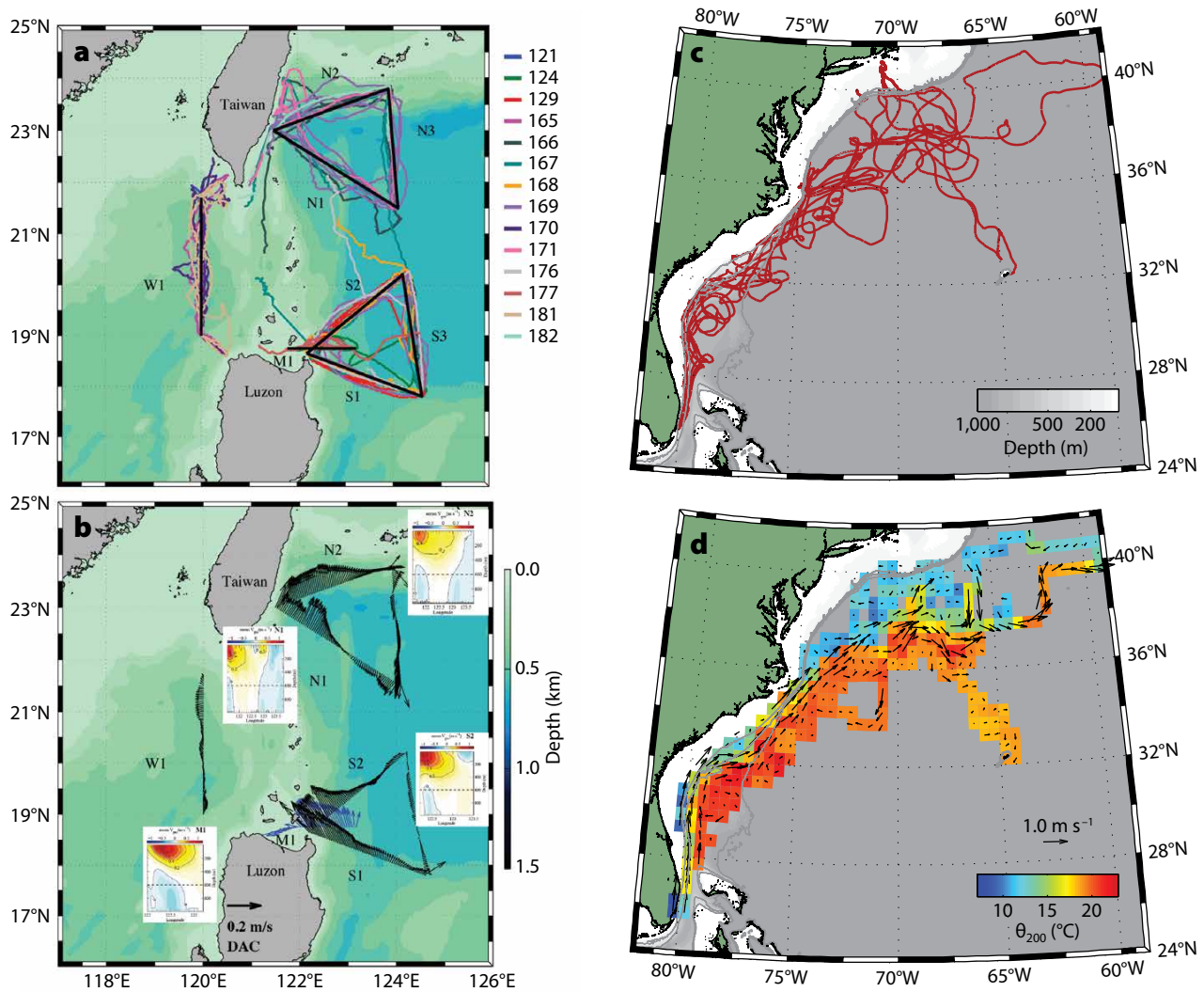
Figure 3. Multiyear glider observations in two mid-latitude western boundary currents. (a) Trajectories from 20 Seaglider missions in the Kuroshio during 2011–2013. (b) Mean depth averaged currents in the upper 1,000 m from gliders (black) and a moored array (blue) and mean cross-track geostrophic currents along select transects (insets). (c) Trajectories of 12 Spray glider missions in the Gulf Stream from 2004–2017. (d) Averages of potential temperature at 200 m and depth averaged currents in 0.5° x 0.5° boxes. (Panels c–d are adapted from Todd, 2017)
