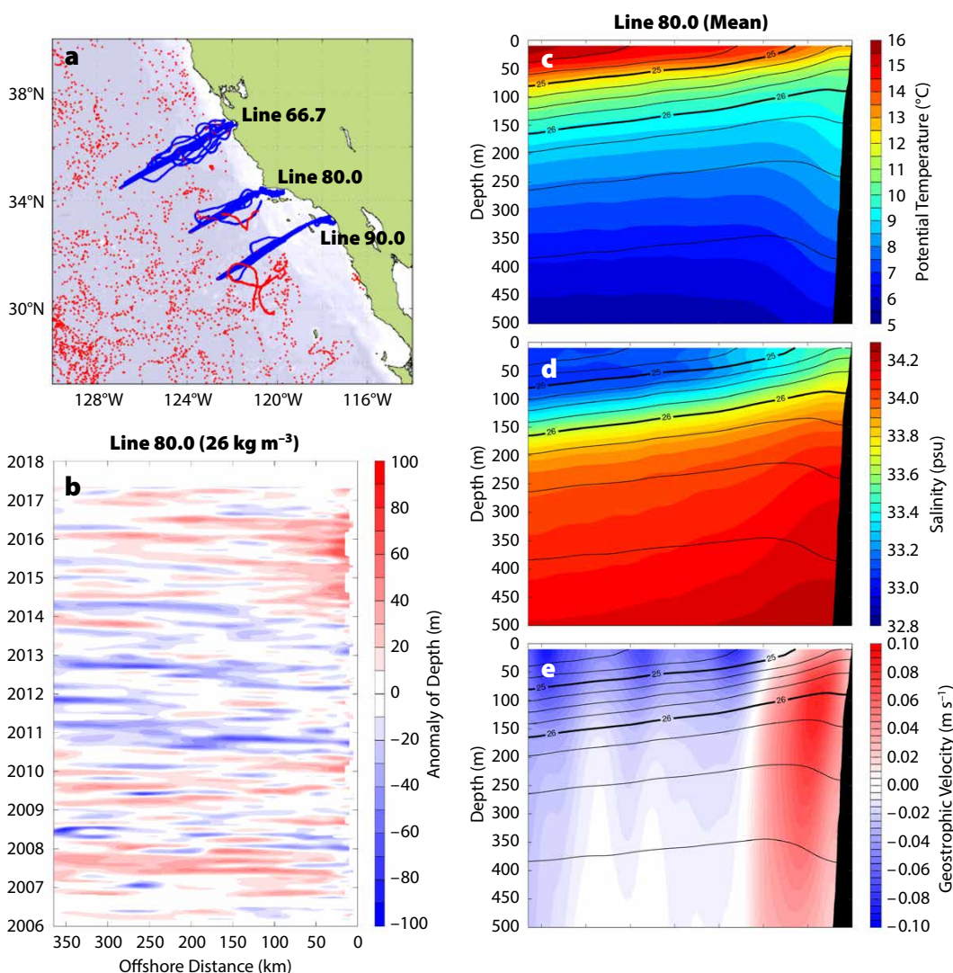
Figure 2. Observations from the California Underwater Glider Network (CUGN). (a) Trajectories of CUGN gliders along CalCOFI Lines 66.7, 80.0, and 90.0 since 2006 (blue) with locations of Argo profiles during the same time period (red). (b) Temporal variability in the depth of the 26 \text{ kg m}^{-3} isopycnal relative to its mean annual cycle along Line 80.0. (c–e) Mean cross-shore transects of (c) potential temperature, (d) salinity, and (e) alongshore geostrophic velocity along Line 80.0. Panels b–e are based on the CUGN climatology of Rudnick et al. (2017) and are available from https://doi.org/10.21238/S8SPRAY7292 .
