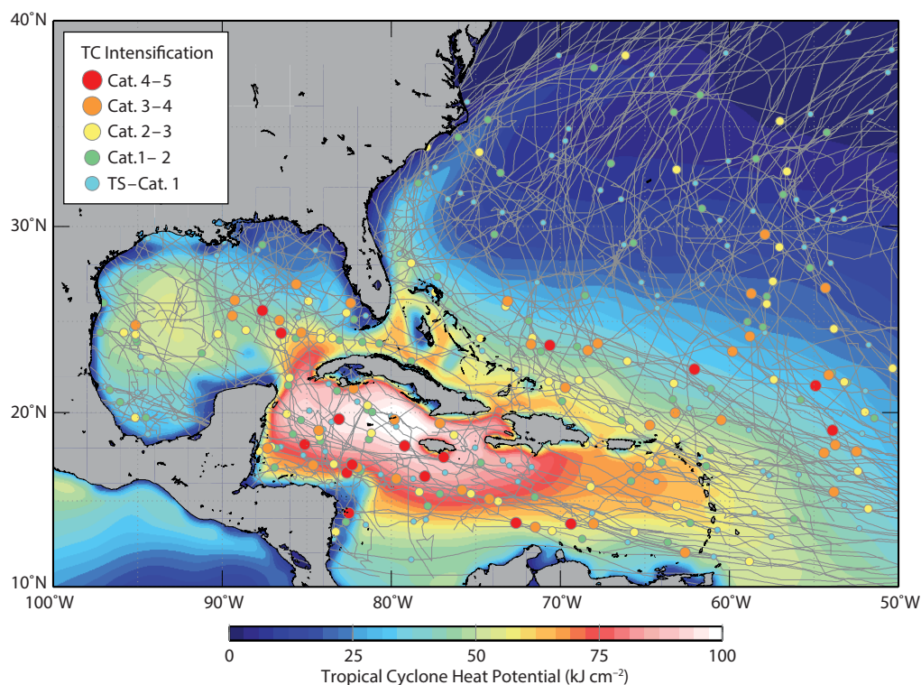
Figure 1. Atlantic hurricane tracks during the period 1993–2010, with color circles indicating the position where they intensified. The background color shows the average Tropical Cyclone Heat Potential during the same period. From Goni et al. (2017)
