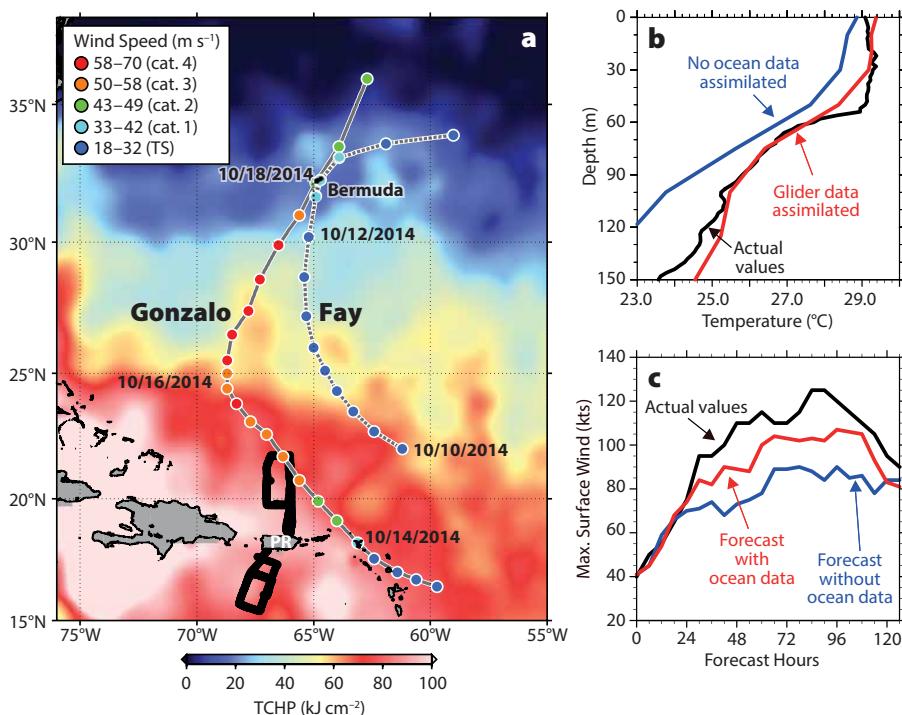
Figure 2. (a) Underwater glider transects (black lines) superimposed to the altimetry-derived upper-ocean heat content (Tropical Cyclone Heat Potential) for mid-October 2014, with Hurricane Gonzalo (2014) and Fay (2014) tracks (circles). (b) Impact of a glider temperature profile in the initialization of HWRf-HYCOM. (c) Impact of glider and other ocean data to reduce error in tropical cyclone intensity (maximum wind speed) during the forecast of Hurricane Gonzalo tested on October 13, 2014. From Goni et al. (2017)
