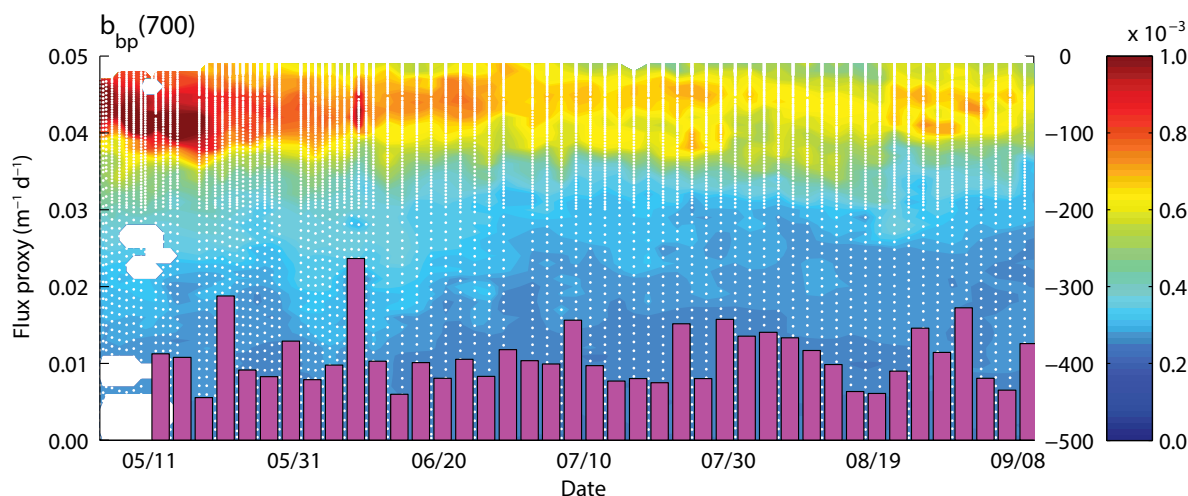
Figure 1. Upper water column optical backscatter (color contours) and particle flux measured at 1,000 m between bio-optical float profiles using an optical sediment trap (magenta bars). Right-hand y-axis denotes depth in meters. Data were collected in 2012 in the western Sargasso Sea. From Estapa et al. (2013)
