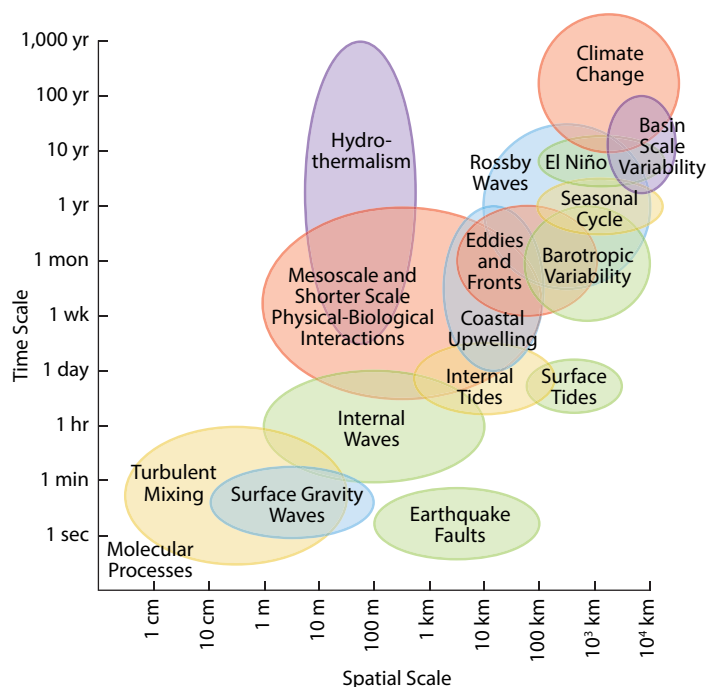
Figure 1. Overlapping spatial and temporal scales of major oceanic processes that are amenable to observation with ALPS. Redrawn from Lampitt et al. (2010)
