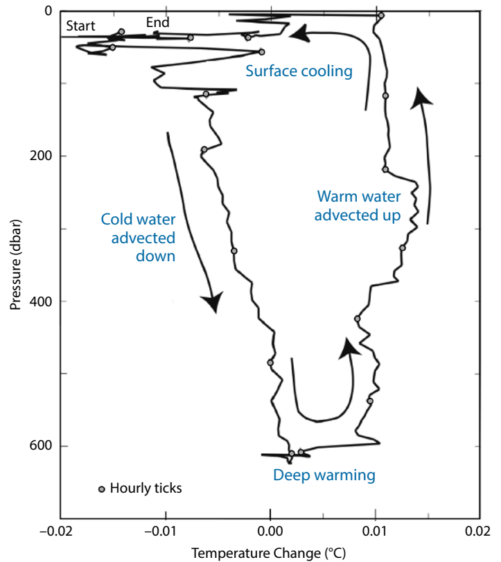
Figure 2. Variation of temperature and depth along a three-dimensional trajectory of a Lagrangian float during deep convection in the Labrador Sea (Steffen and D'Asaro, 2002) illustrate the cycle of warming and cooling that drives the convection. Water parcels cool and become heavier at the surface and thus sink, carrying cold water downward and warming slightly by mixing with the surrounding water. At about 600 m depth, they encounter warmer, saltier water at the bottom of the convective layer, and warm by mixing with this water. They then move upward, carrying warmer water, until they reach the surface to repeat the cycle.
