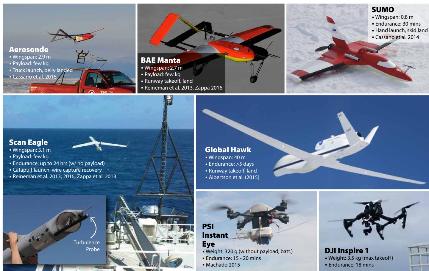
Figure 1. Examples of unmanned aerial vehicles presently used for oceanographic or atmospheric research, with sample studies referenced.
