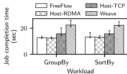
Figure 16: Spark performance on FreeFlow .
