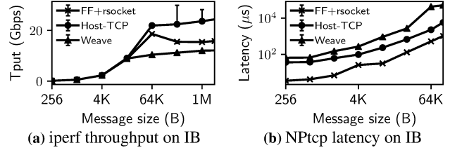
Figure 14: TCP throughput and latency between a pair of containers on different hosts. We compare native TCP with FreeFlow + rsocket (socket-to-Verbs translation).
