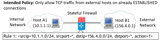
Figure 1: Network set-up
