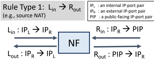
Figure 14: NAT example
