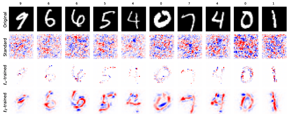
(a) MNIST
