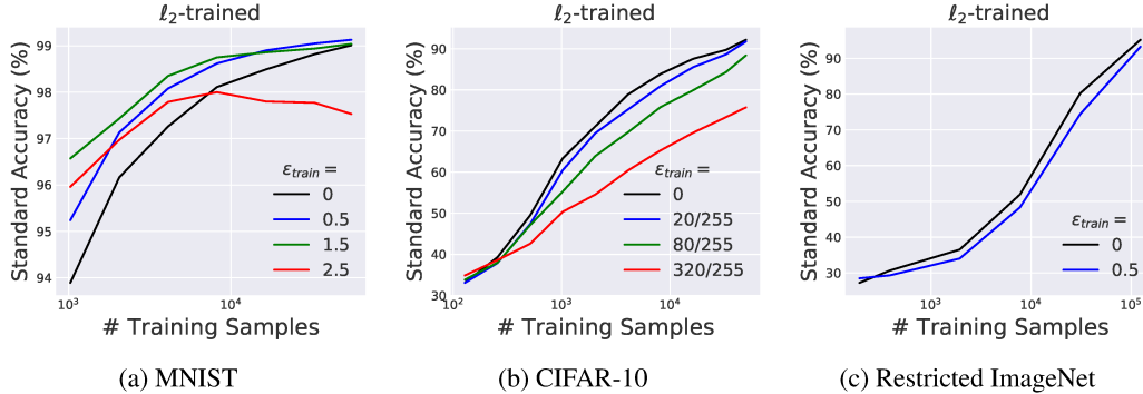
Figure 1: Comparison of the standard accuracy of models trained against an \ell_2 -bounded adversary as a function of size of the training dataset. We observe that when training with few samples, adversarial training has a positive effect on model generalization (especially on MNIST). However, as training data increase, the standard accuracy of robust models drops below that of the standard model ( \epsilon_{train} = 0 ). Similar results for \ell_\infty trained networks are shown in Figure 6 of Appendix G.
